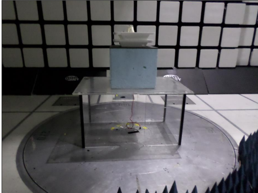
Photograph 7. Radiated Emissions, >1 GHz Scan, Front
