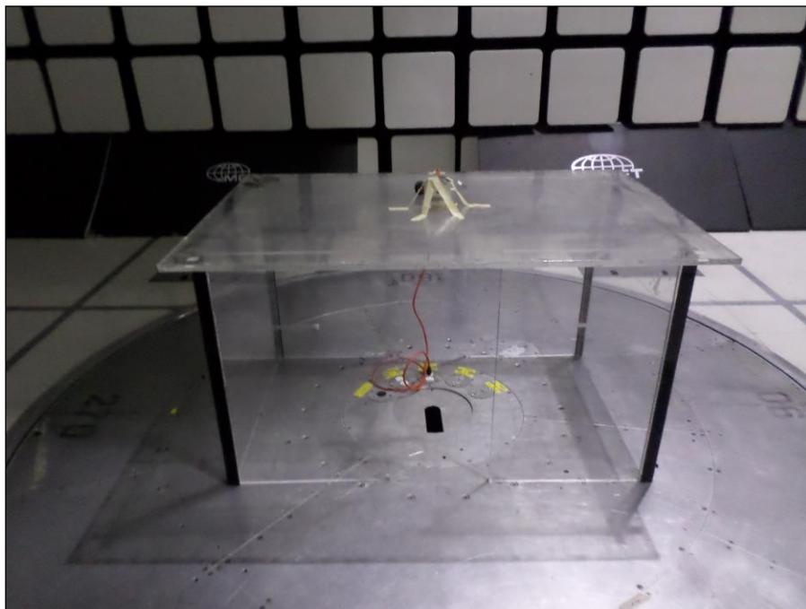
Photograph 4. Radiated Emissions, Front
