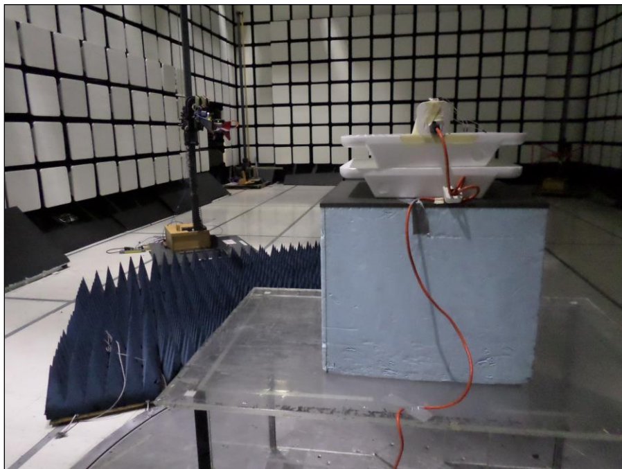
Photograph 8. Radiated Emissions, >1 GHz Scan, Rear
