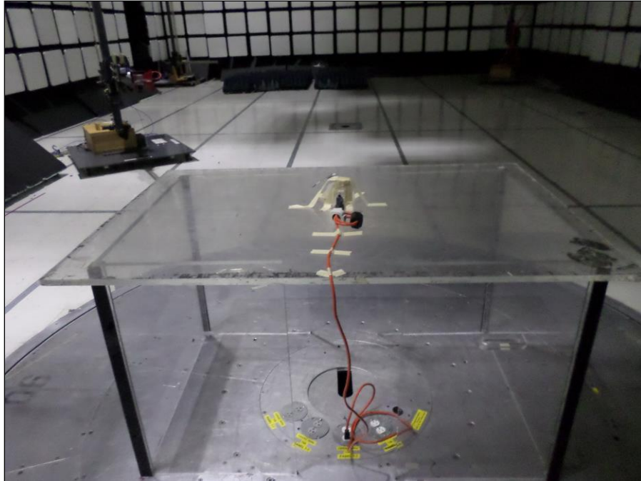
Photograph 5. Radiated Emissions, Rear
