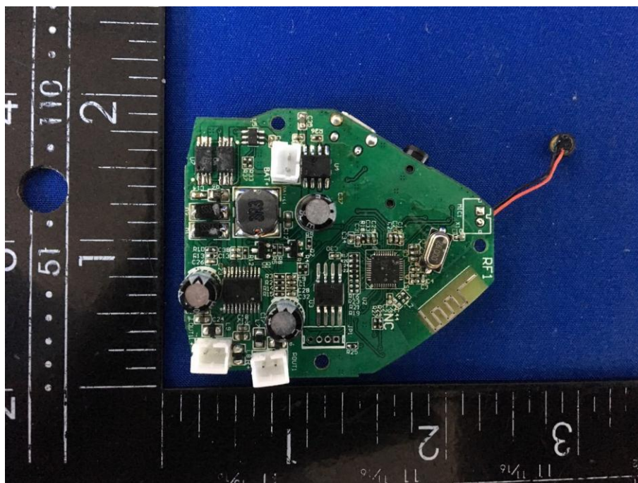
Mainboard-Rear View
