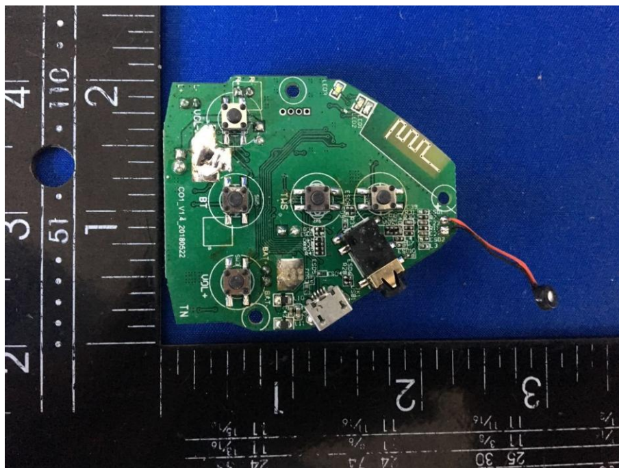
Mainboard-Front View
