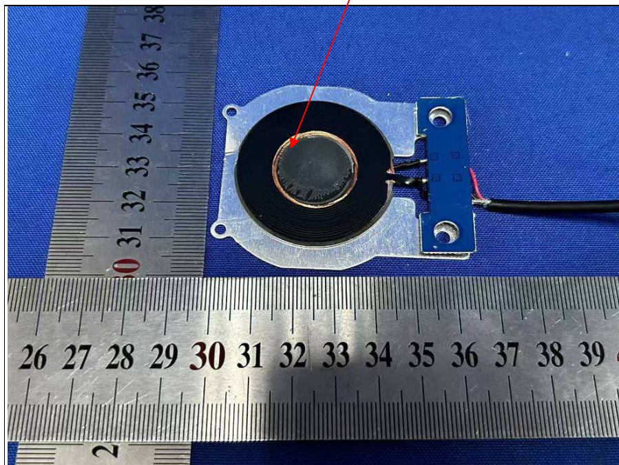
25W Coil ANT.
