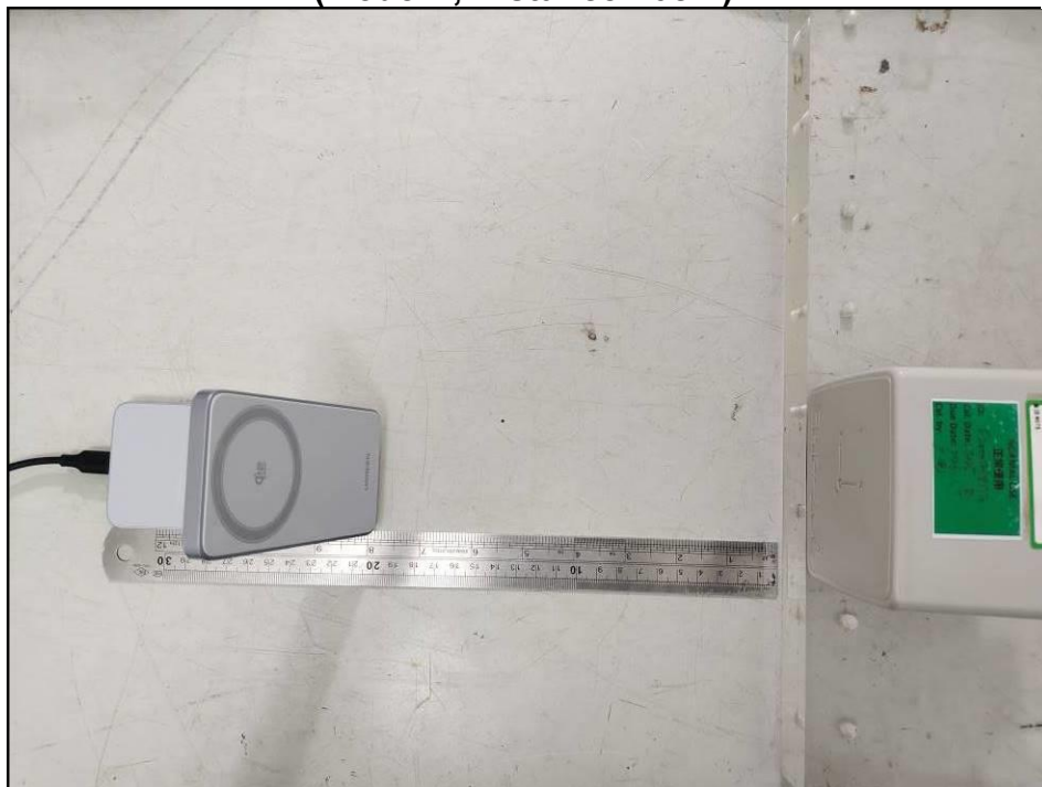
Magnetic & Electric Field (Mode A, Distance:15cm)
