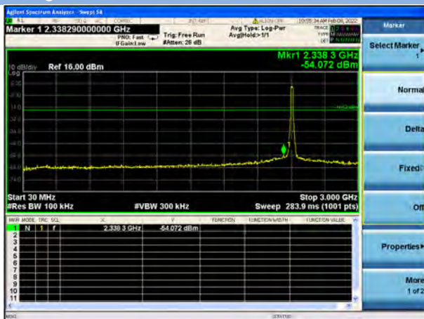
802.11g CHANNEL 1, SPURIOUS 30 MHz ~ 3 GHz
