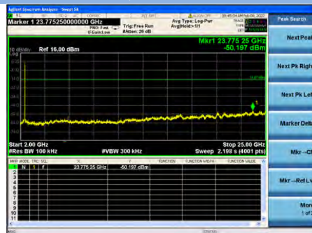
802.11b CHANNEL 5, SPURIOUS 2 GHz ~ 25 GHz
