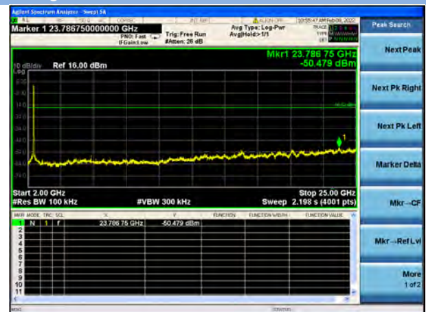
802.11g CHANNEL 1, SPURIOUS 2 GHz ~ 25 GHz
