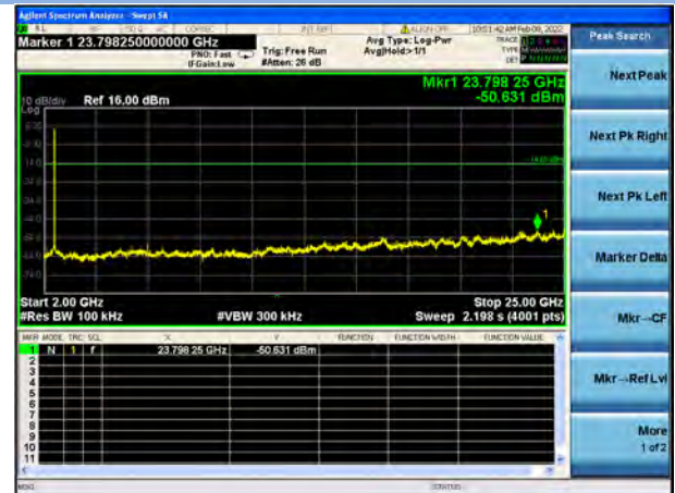
802.11b CHANNEL 11, SPURIOUS 2 GHz ~ 25 GHz
