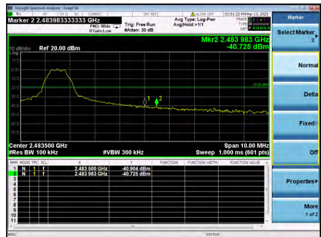
GFSK (BLE 1Mbps) HIGH CHANNEL, BAND EDGE
