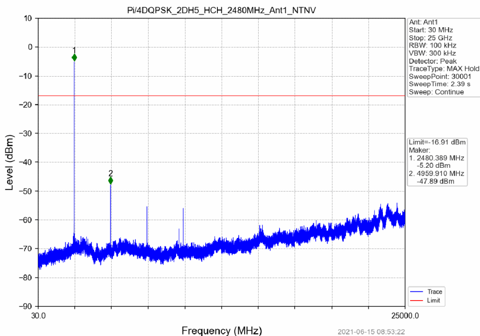
\pi /4-DQPSK_2DH5_HCH_2480MHz_Ant1_NTNV
