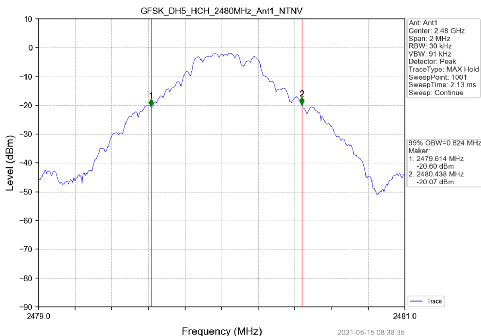
GFSK_DH5_HCH_2480MHz_Ant1_NTNV
