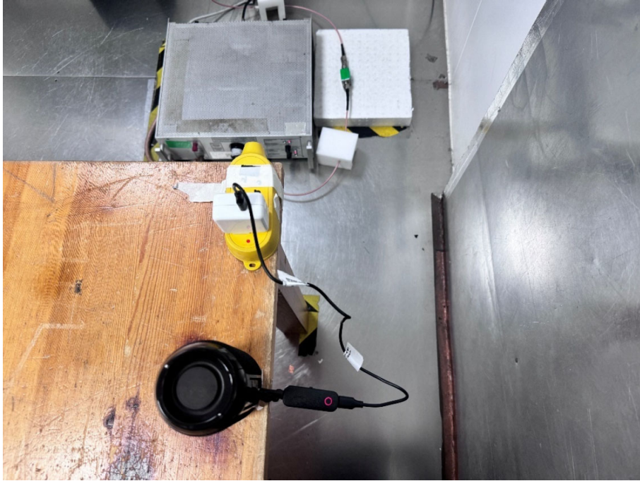
Photo 4-RX Mode
