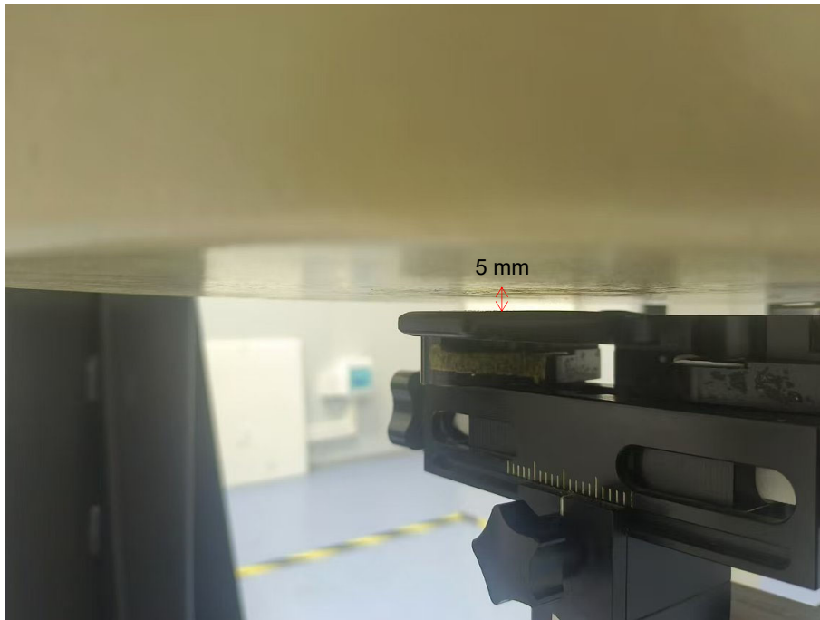
Horizontal-Up (5mm)
