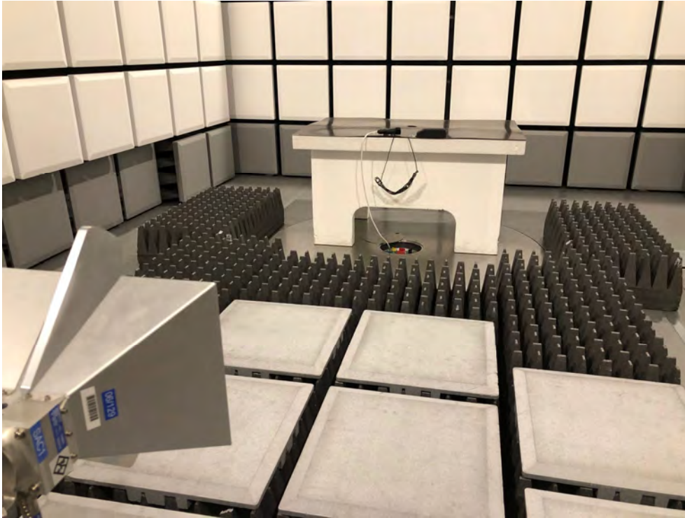
Figure 8: Radiated emission test
