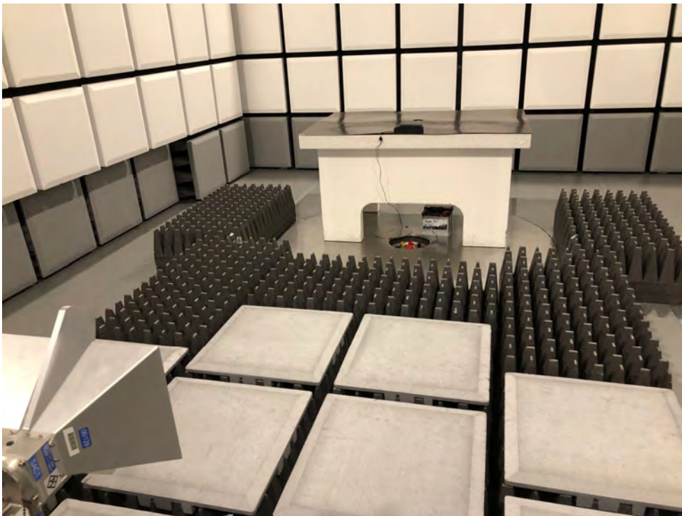
Figure 9: Radiated emission test
