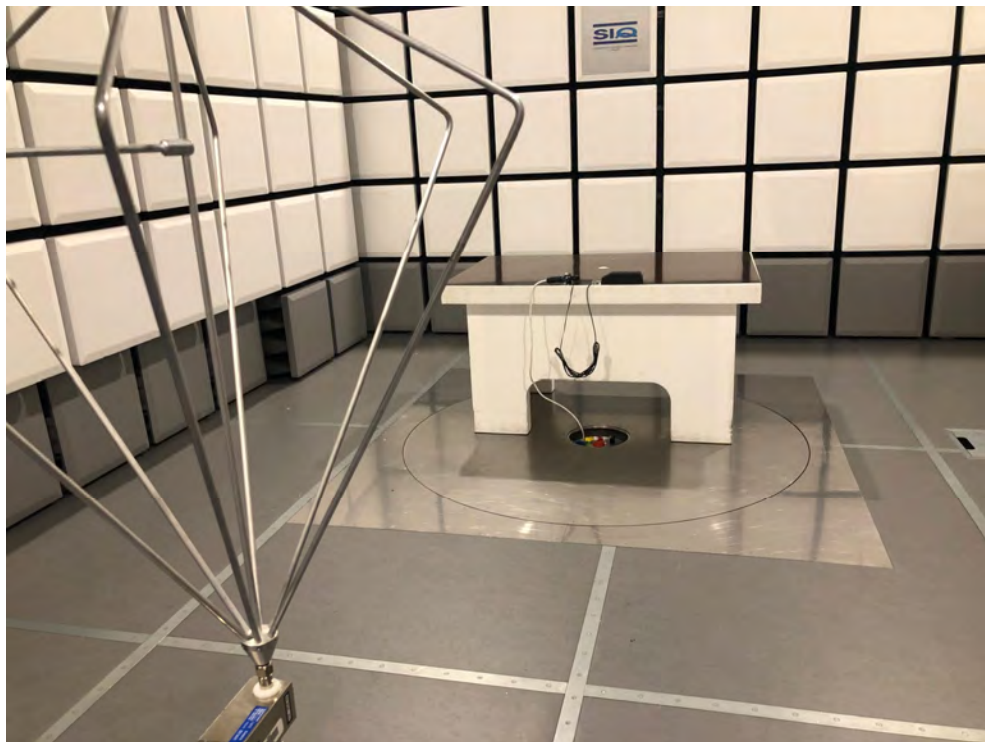
Figure 2: Radiated emission test
