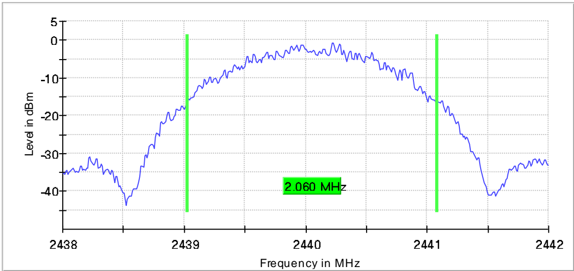
99 % Bandwidth
