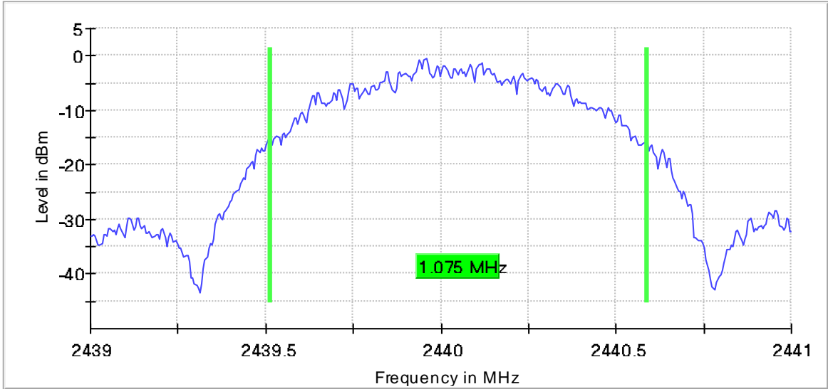
99 % Bandwidth
