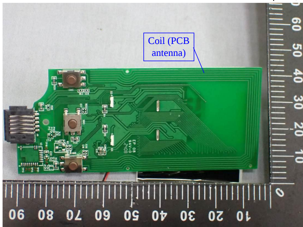
Figure 14 Internal View (PCB, Back View)
