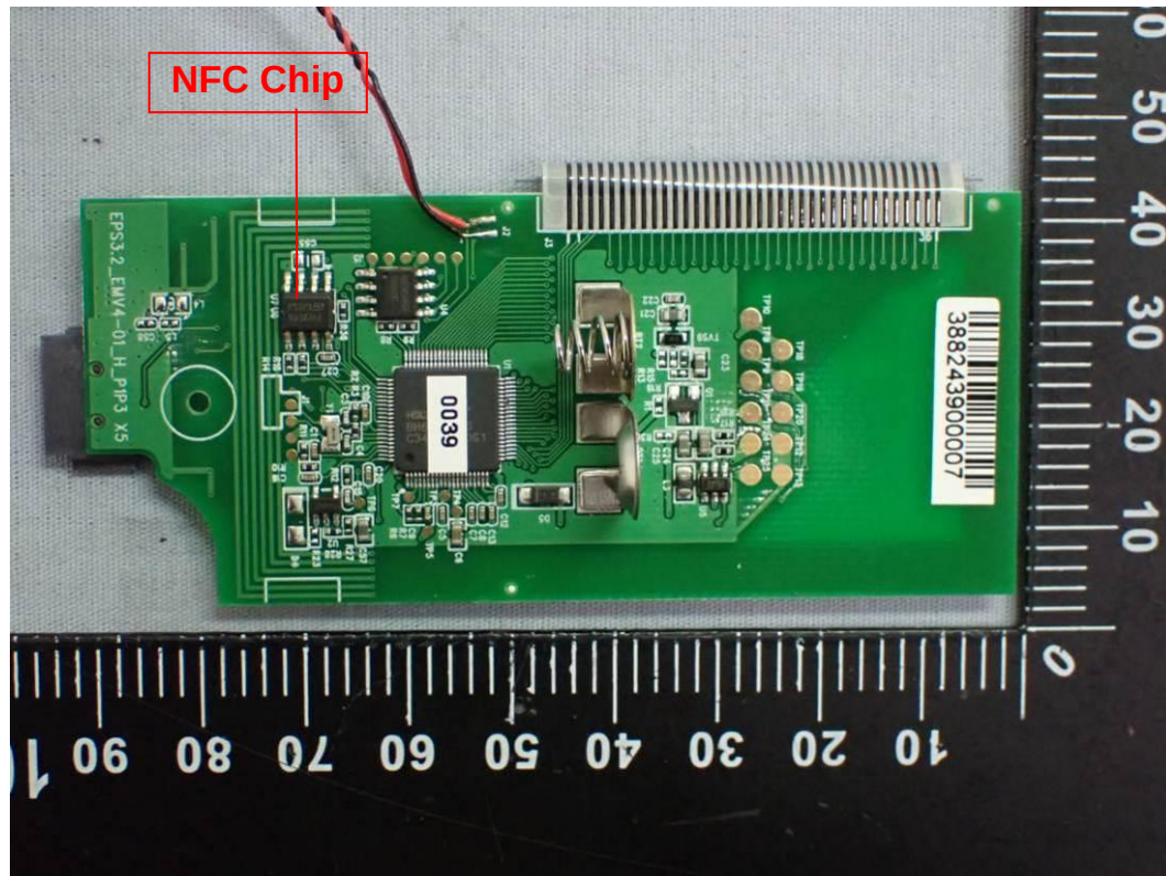
Figure 13 Internal View (PCB, Front View)
