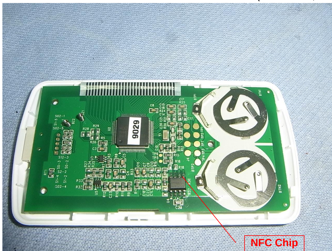
Figure 9 Internal View (PCB Board, Front View)
