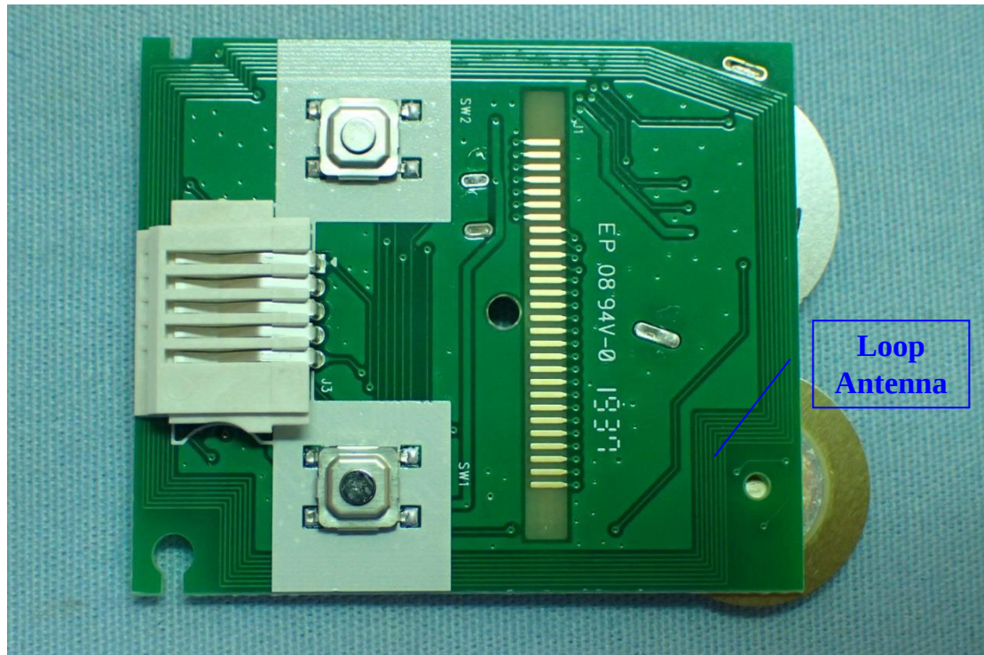
Figure 5 Internal View (Control Board, Back View)
