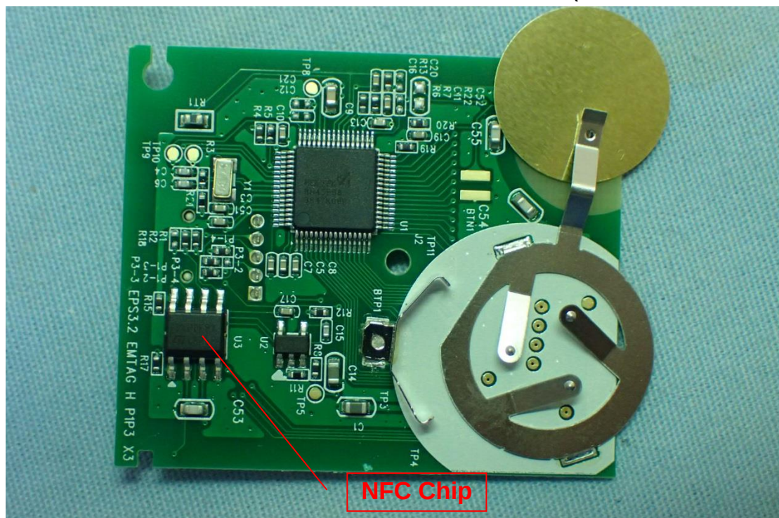
Figure 6 Internal View (Control Board, Front View)
