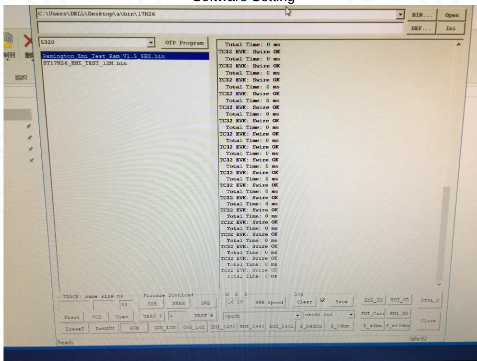
Software Setting
