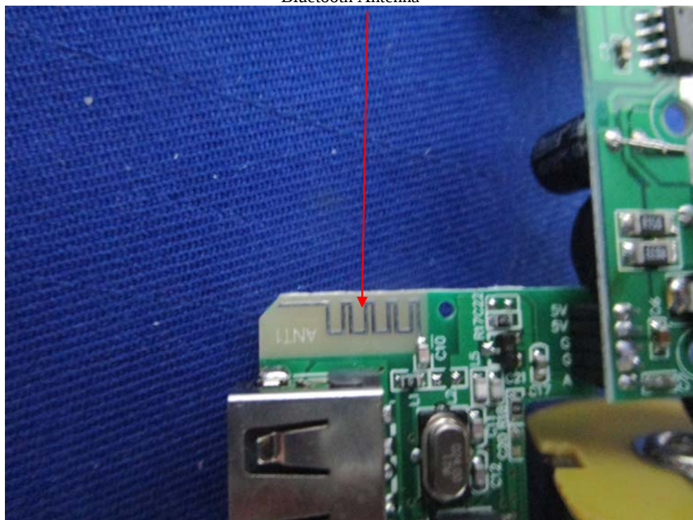
Bluetooth Antenna
