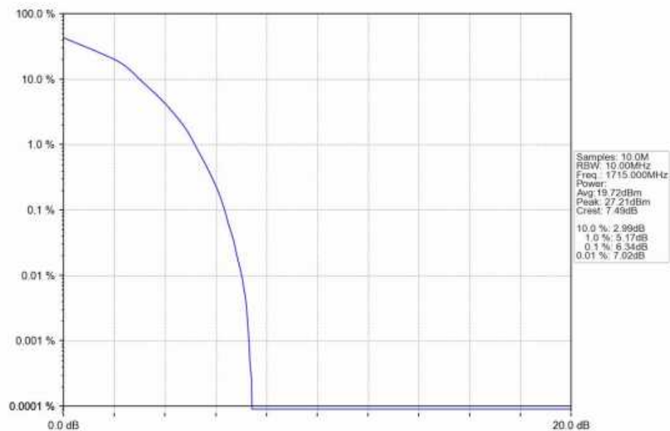
Band66_10MHz_16QAM_LCH_1715MHz_RB_27_0_NTNV
