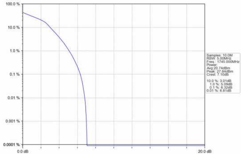
Band66_3MHz_16QAM_MCH_1745MHz_RB_15_0_NTNV
