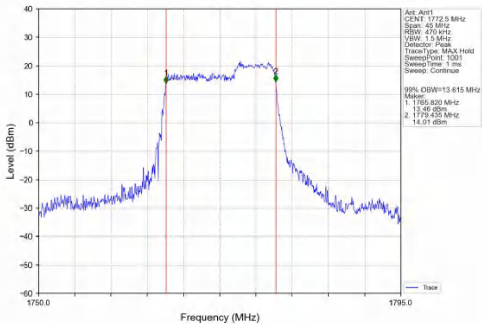
Band66_15MHz_16QAM_HCH_1772.5MHz_RB_27_48_NTNV
