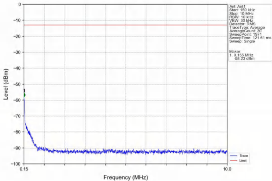
Band66_5MHz_QPSK_MCH_1745MHz_RB_1_0_NTNV
