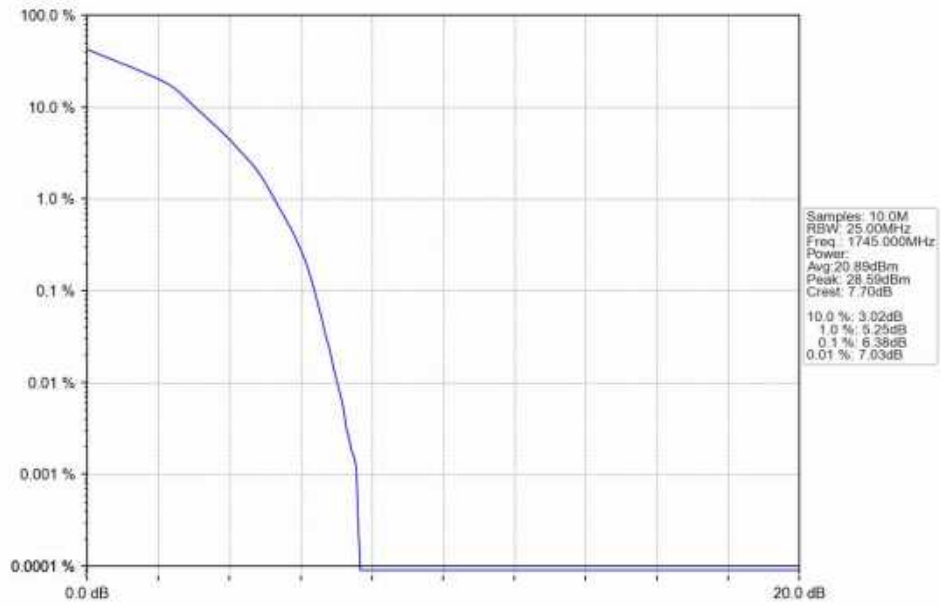
Band66_20MHz_16QAM_MCH_1745MHz_RB_27_0_NTNV
