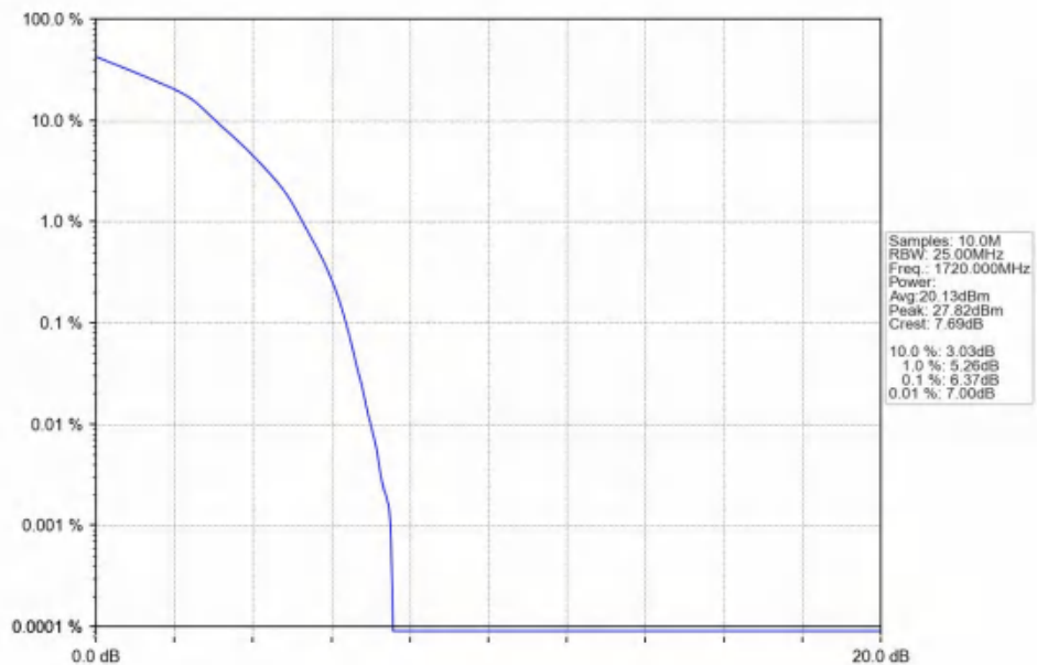
Band66_20MHz_16QAM_LCH_1720MHz_RB_27_0_NTNV
