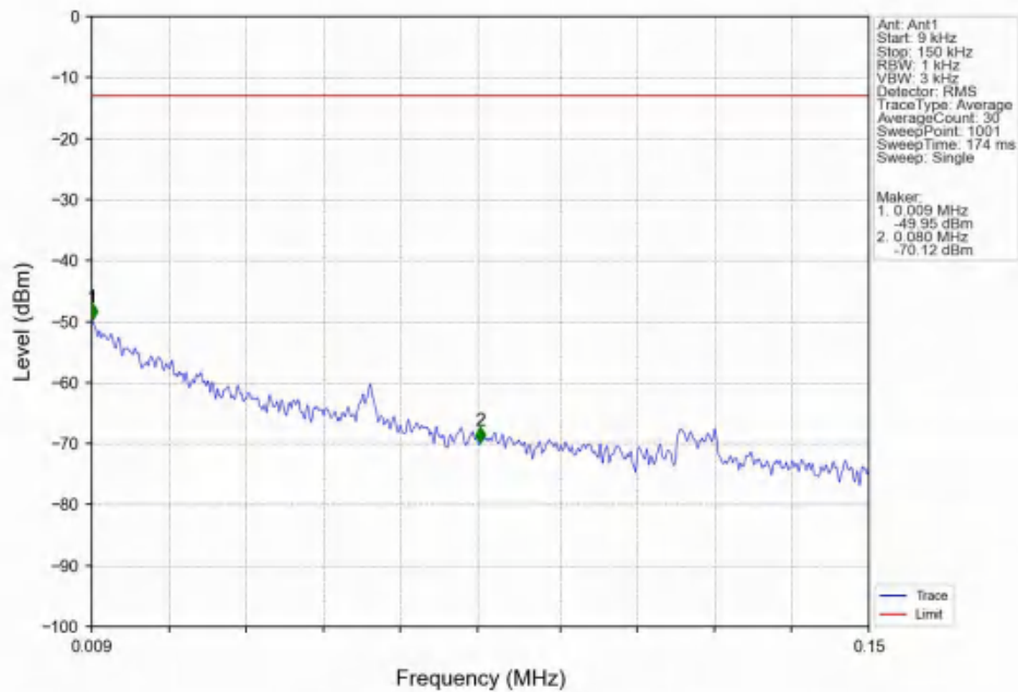
Band66_5MHz_16QAM_LCH_1712.5MHz_RB_1_0_NTNV
