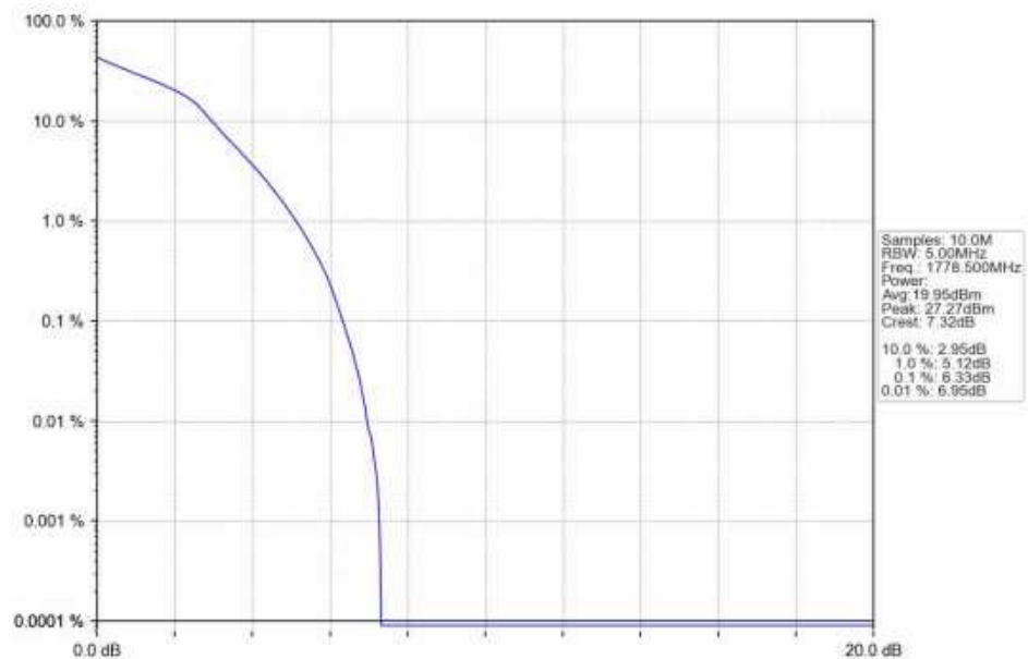
Band66_3MHz_16QAM_HCH_1778.5MHz_RB_15_0_NTNV
