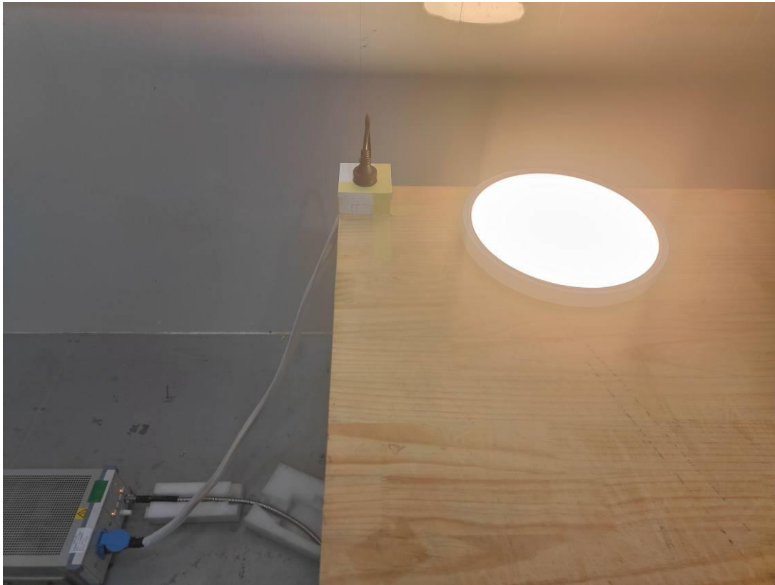
AC Line Conducted Emission
