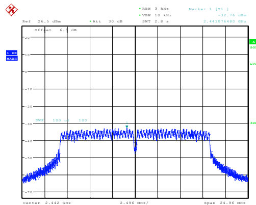
g_2442MHz_Chain 0 -32.76dBm/3kHz
