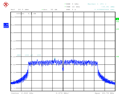
n20_2442MHz_Chain 0 -33.81dBm/3kHz
