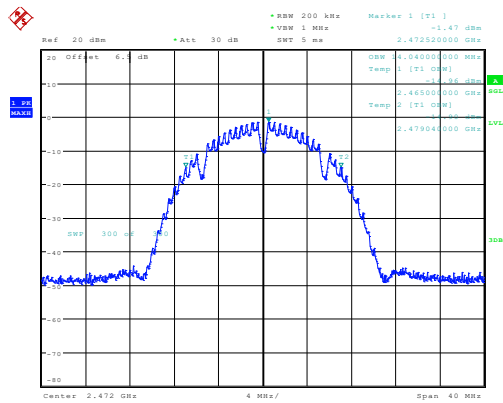
b_2472MHz_Chain 0 14.040MHz
