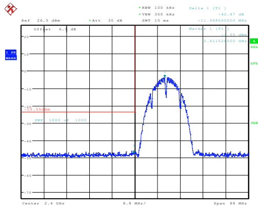
b_2412MHz_Chain 0 42.47dB
