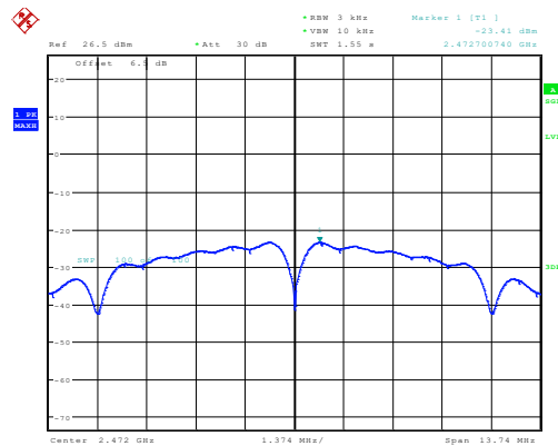
b_2472MHz_Chain 0 -23.41dBm/3kHz
