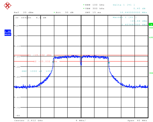
g_2412MHz_Chain 0 16.640MHz
