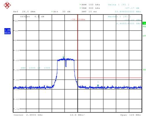
g_2472MHz_Chain 0 27.17dB
