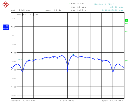
b_2412MHz_Chain 0 -23.68dBm/3kHz
