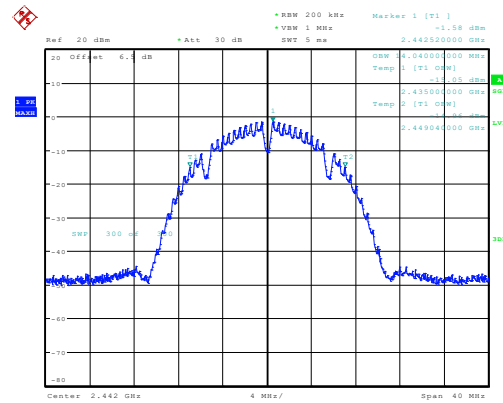
b_2442MHz_Chain 0 14.040MHz
