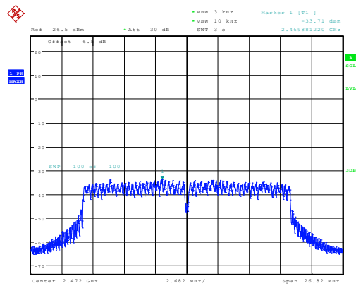
n20_2472MHz_Chain 0 -33.71dBm/3kHz
