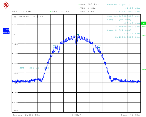
b_2412MHz_Chain 0 14.040MHz
