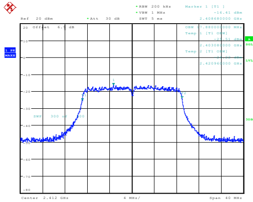
n20_2412MHz_Chain 0 17.880MHz
