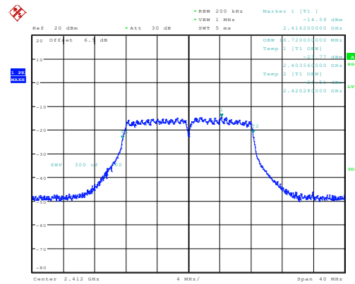
g_2412MHz_Chain 0 16.720MHz
