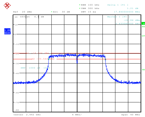
n20_2442MHz_Chain 0 17.840MHz
