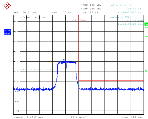
n20_2472MHz_Chain 0 24.42dB
