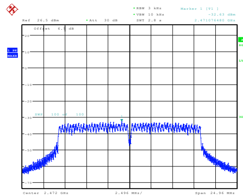
g_2472MHz_Chain 0 -32.63dBm/3kHz
