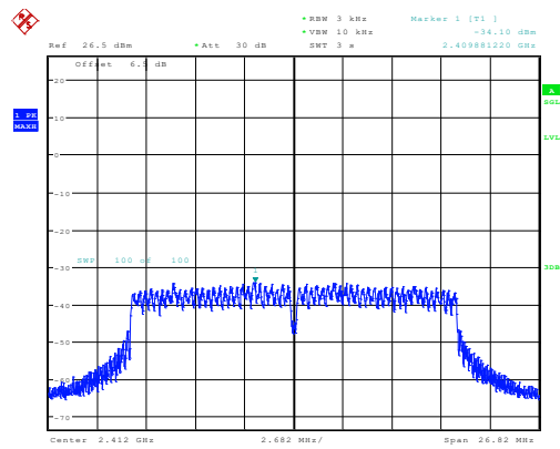
n20_2412MHz_Chain 0 -34.10dBm/3kHz
