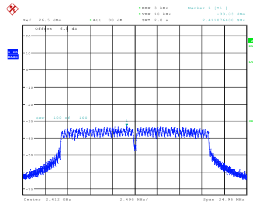
g_2412MHz_Chain 0 -33.03dBm/3kHz
