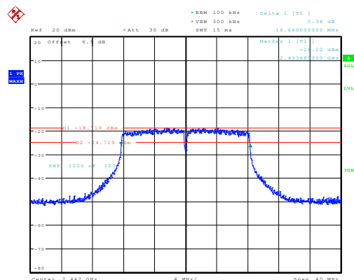
g_2442MHz_Chain 0 16.640MHz
