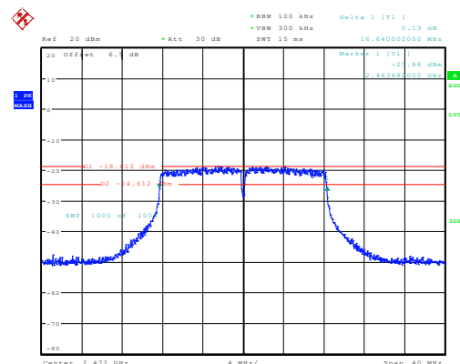
g_2472MHz_Chain 0 16.640MHz
