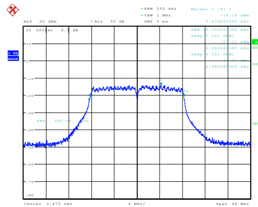
g_2472MHz_Chain 0 16.720MHz
