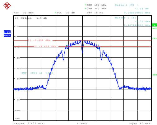
b_2472MHz_Chain 0 9.160MHz
