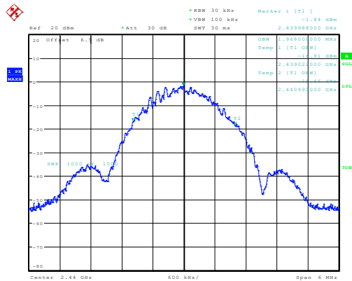
Middle 1.968MHz
