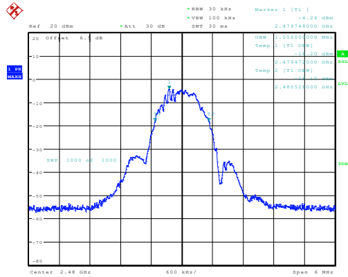
High 1.056MHz
