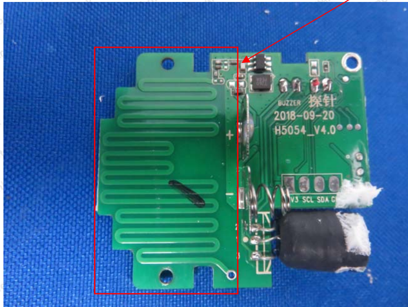
PCB Antenna
