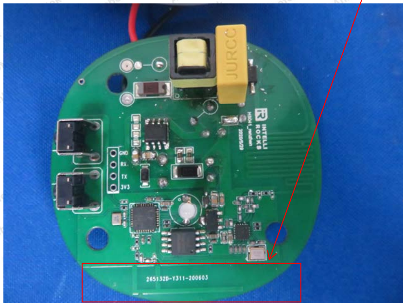
WIFI Antenna
