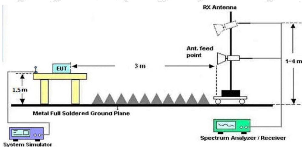
Figure 3. Above 1 GHz
