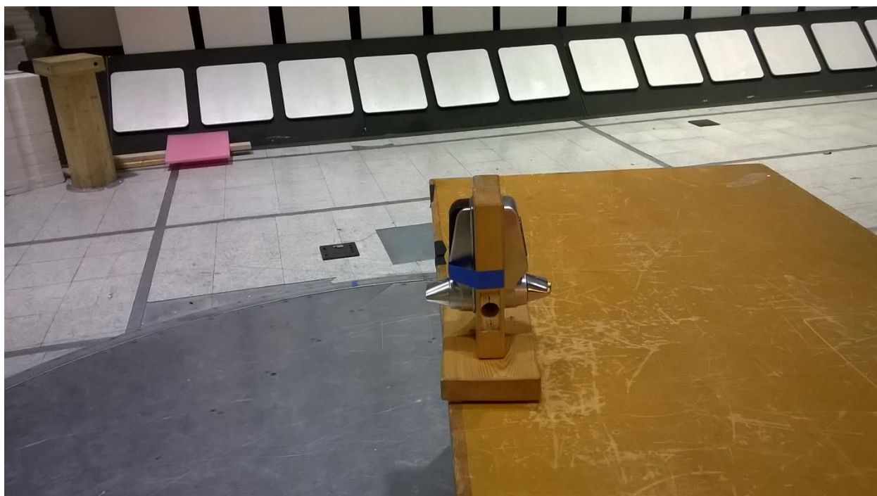
Figure 3 – 30 MHz – 1 GHz, additional absorber on floor was NOT used
