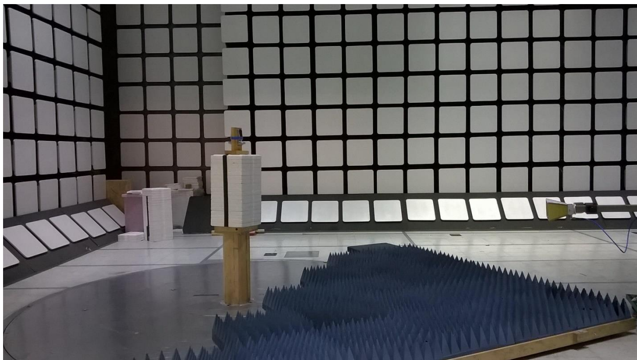
Figure 2 – 1 GHz – 24 GHz, additional absorber on floor WAS used
