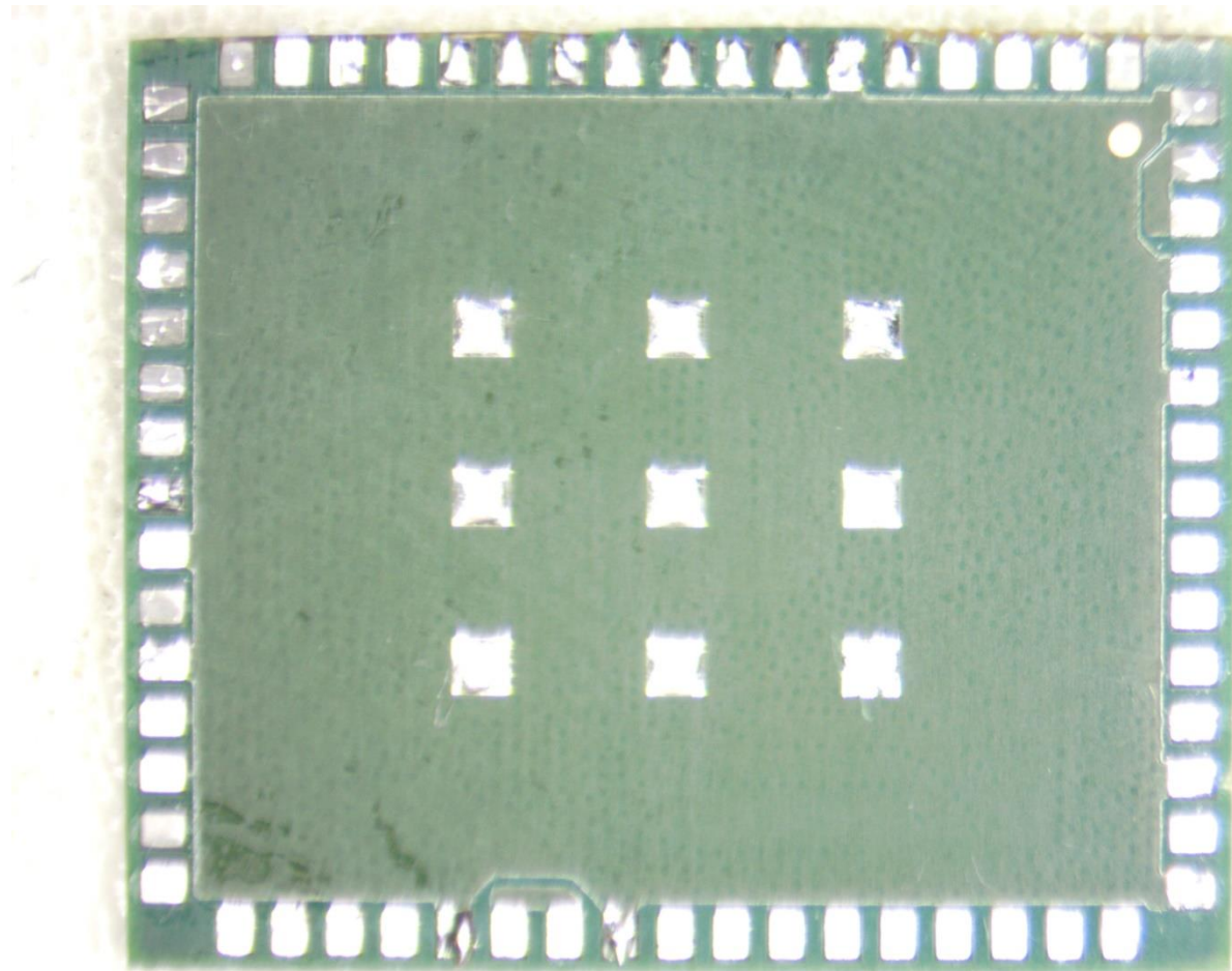
Figure 10 - Back of module
