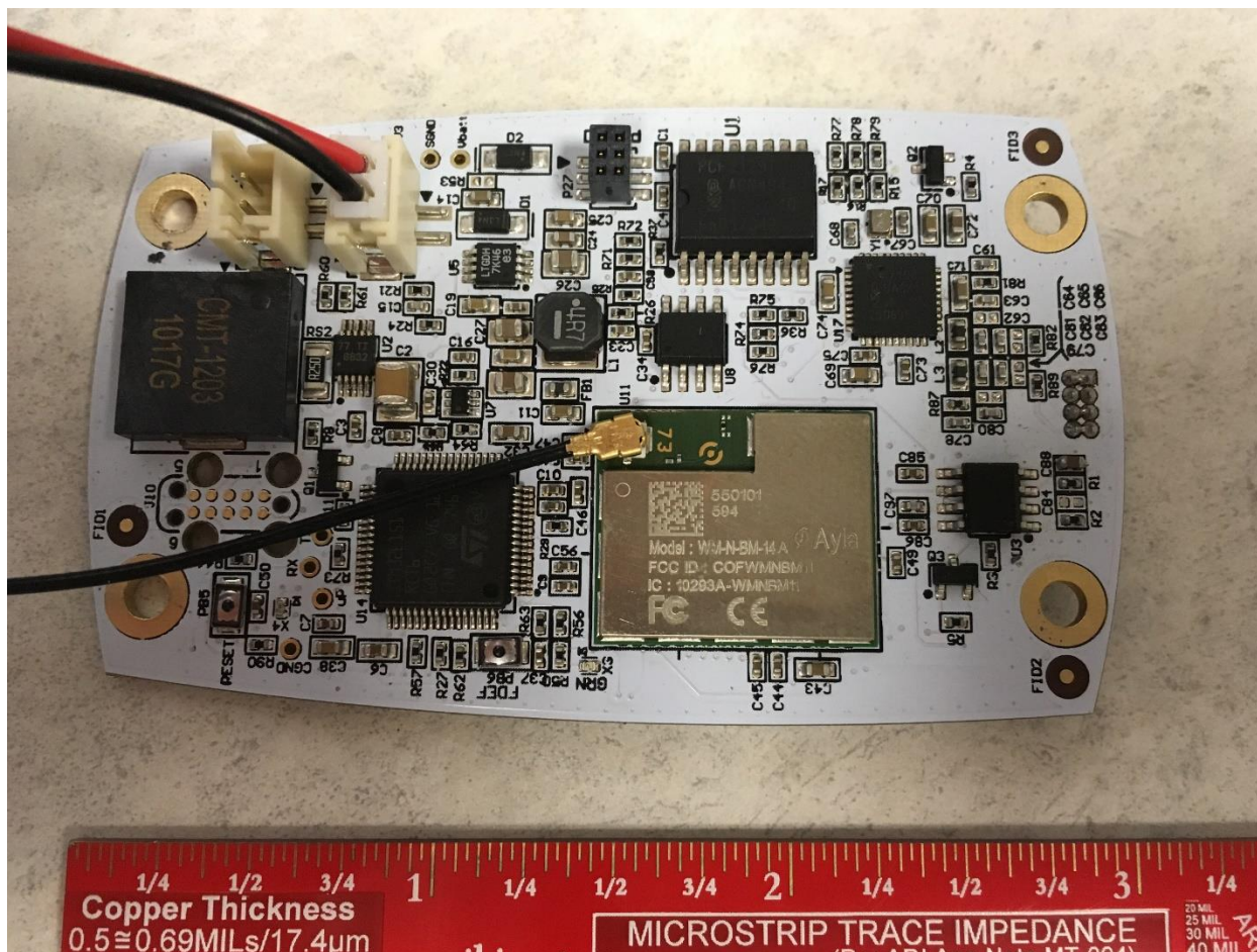
Figure 1 - Main PCB, located under keypad
