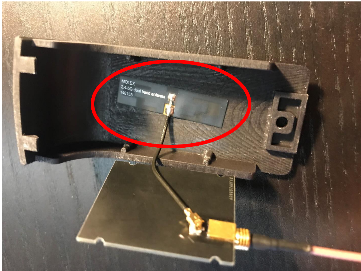
Red circle indicates location of antenna. This is inside the battery access compartment.
