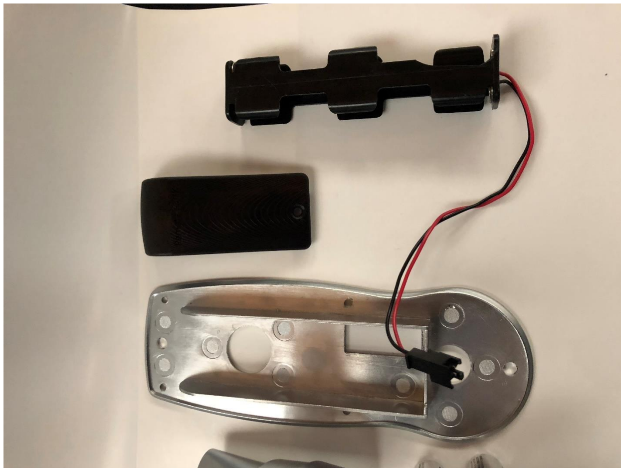
Figure 5 - Battery side of lock disassembled
