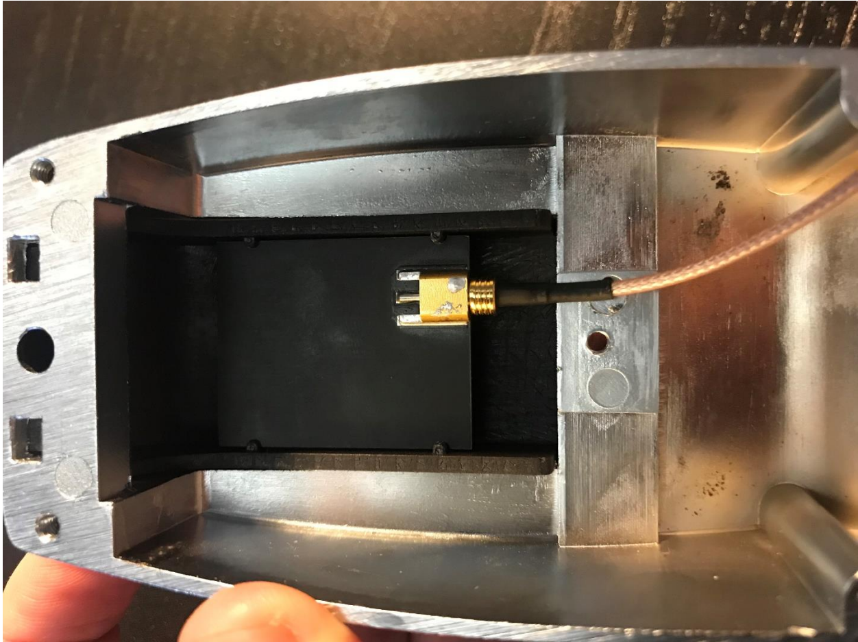
Figure 6 - Battery side of lock disassembled Battery compartment with battery removed
