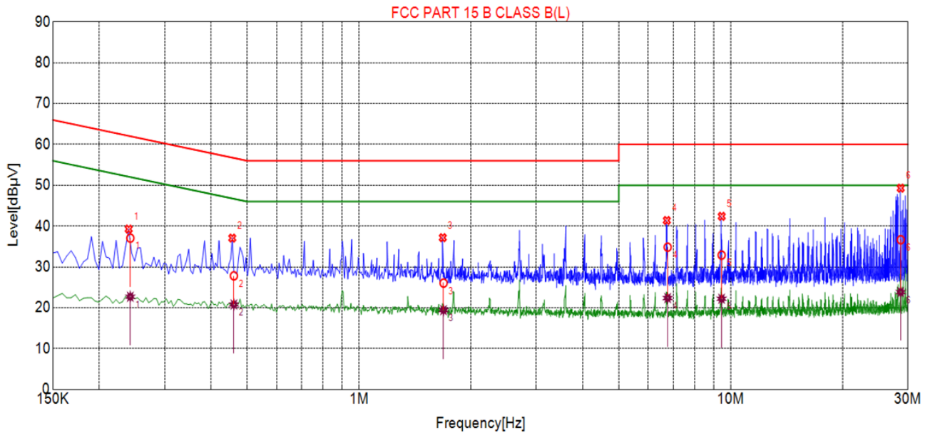
Line Conducted Emission Test Line 1-L
