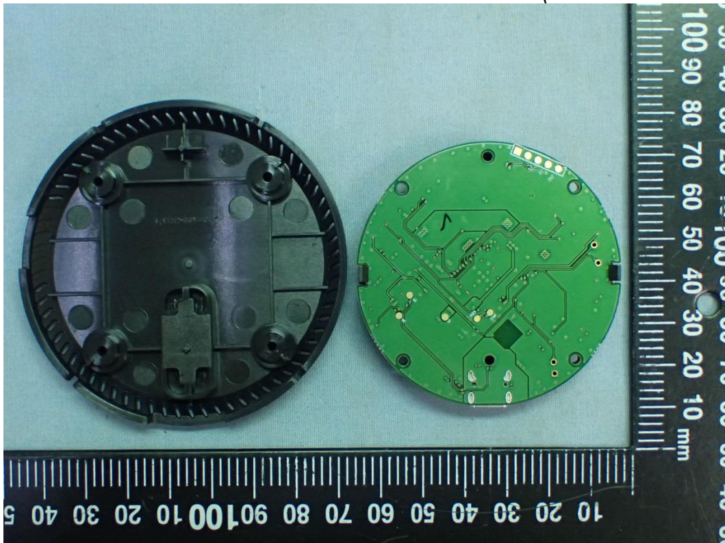
Figure 11 Internal View (Removed Main Board)
