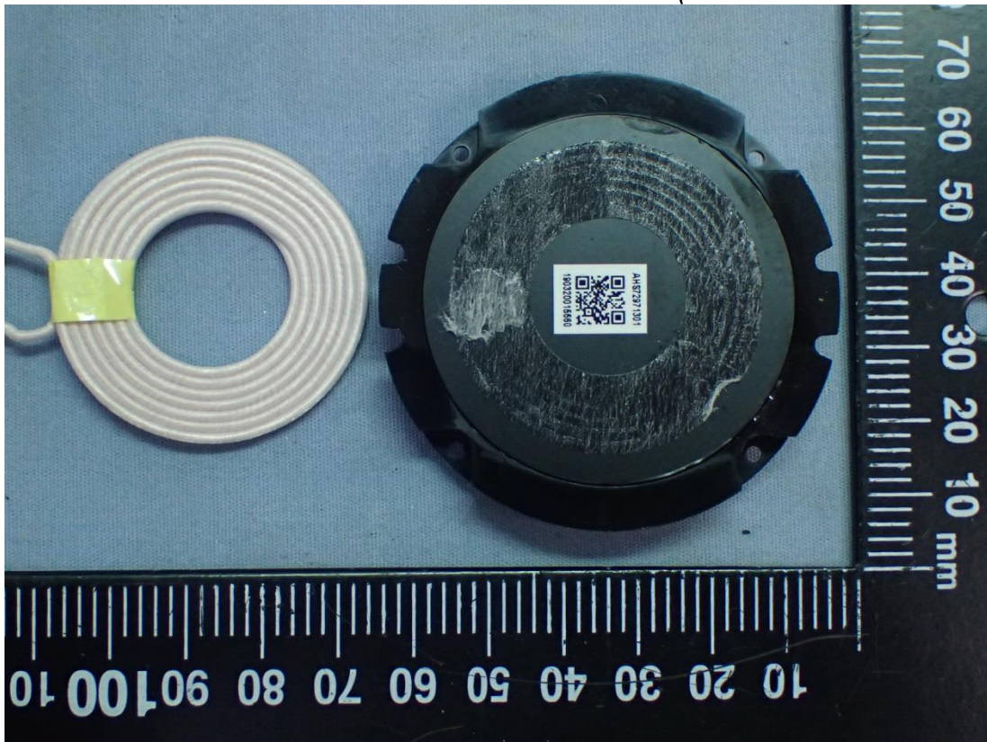
Figure 14 Internal View (Removed WPC Antenna)
