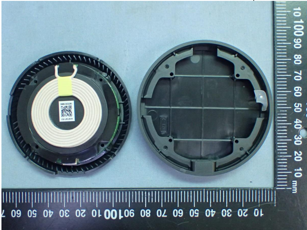
Figure 10 Internal View (Removed Cover)
