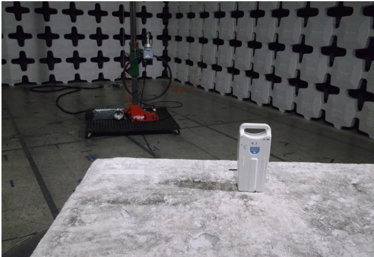
Test Configuration Photographs (Radiated Emissions - Below 30 MHz)
