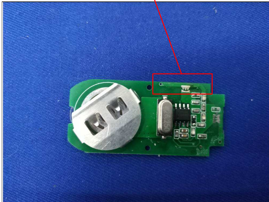
315MHz Antenna
