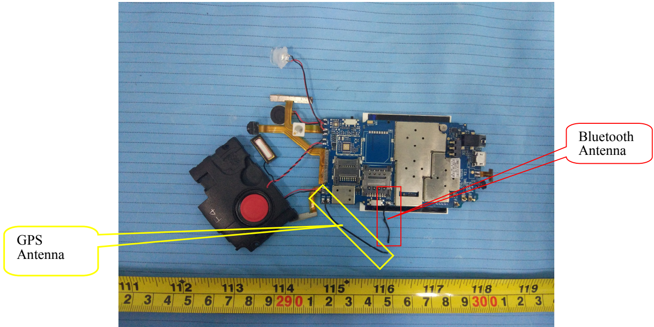
EUT – Main Board Bottom View
