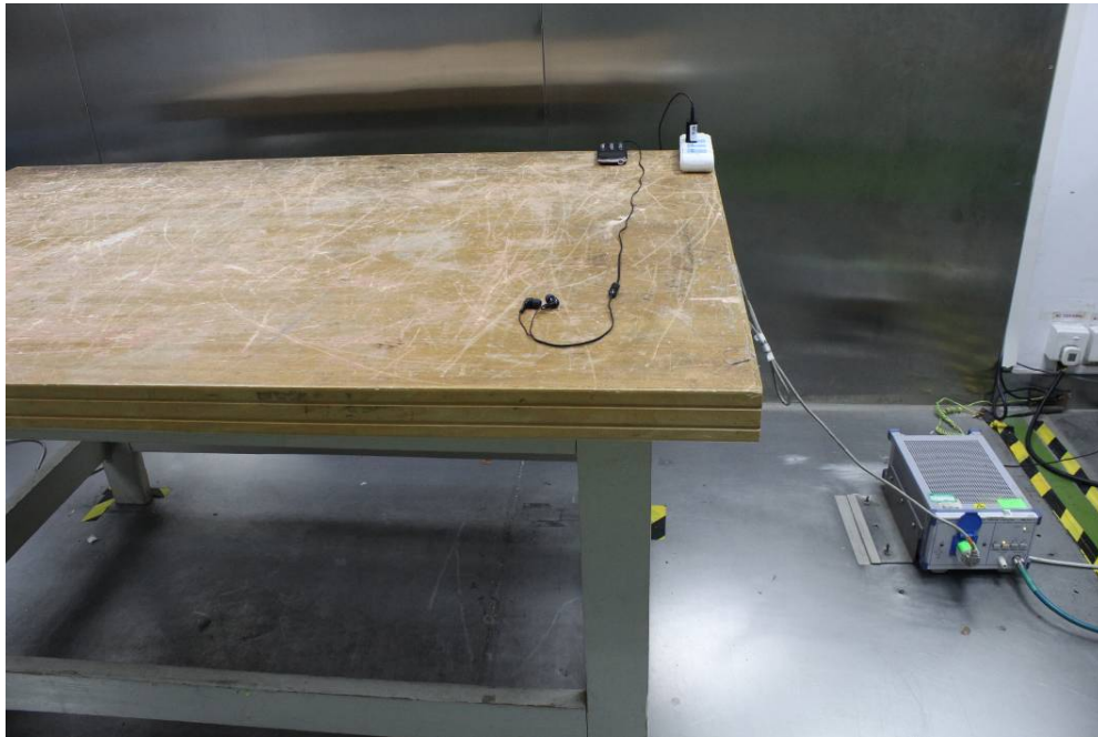
Conducted Emissions - Front View (Charging by Adapter)
