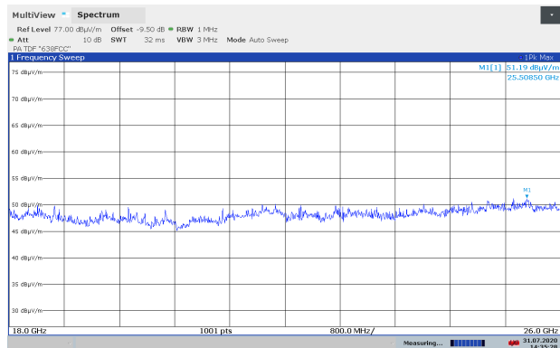
Emissions 18-26 GHz, Ch157, 802.11a 6M, Ant1, VP, @1m
