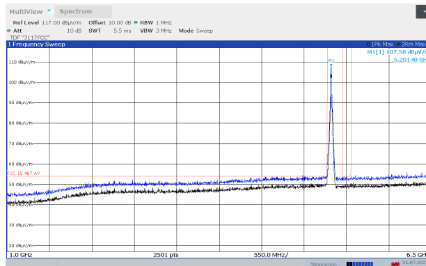
Radiated Emissions 1-6.5 GHz, Ch040, 802.11n HT20, EUT V, Ant 1, VP
