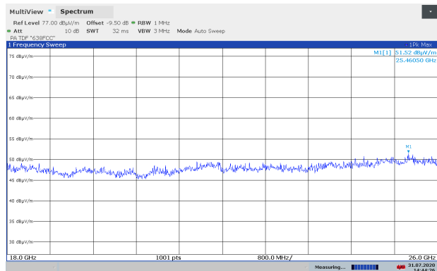
Emissions 18-26 GHz, Ch112, 802.11n HT20, Ant2, VP, @1m
