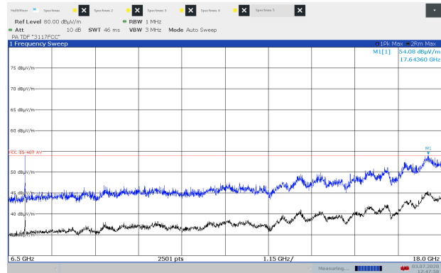
Radiated Emissions 6.5-18 GHz, Ch040, 802.11n HT20, EUT V, Ant 2, VP
