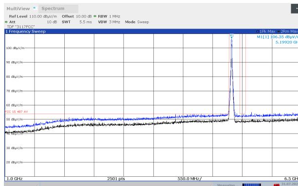
Radiated Emissions 1-6.5 GHz, Ch040, 802.11n HT20, EUT V, Ant 2, VP
