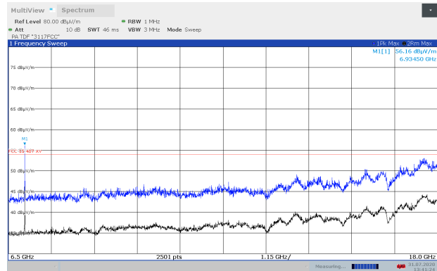
Radiated Emissions 6.5-18 GHz, Ch040, 802.11n HT20, EUT V, Ant 1, VP
