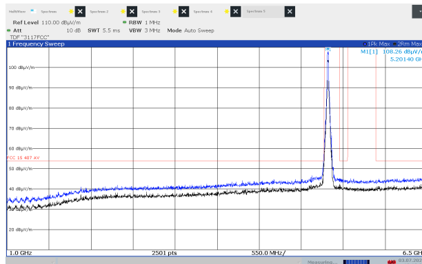
Radiated Emissions 1-6.5 GHz, Ch040, 802.11a 6M, EUT V, Ant 2, VP
