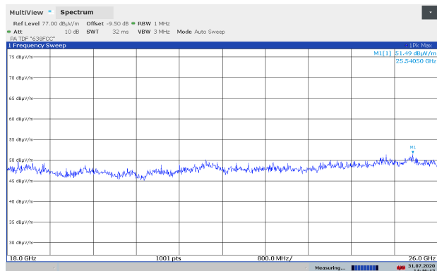
Emissions 18-26 GHz, Ch112, 802.11n HT20, Ant1, VP, @1m
