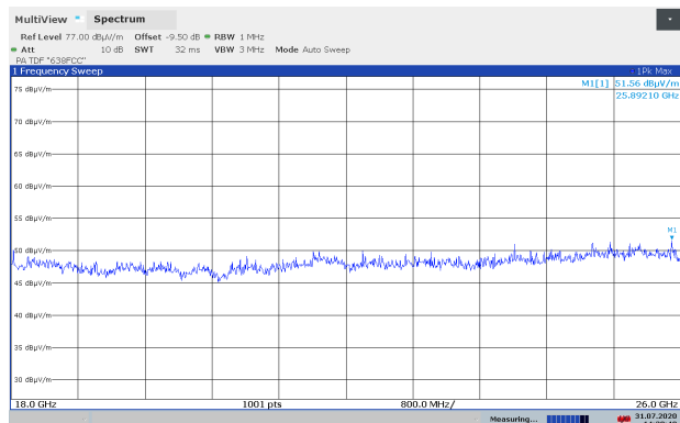
Emissions 18-26 GHz, Ch157, 802.11a 6M, Ant2, VP, @1m
