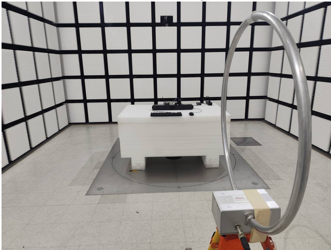
Radiated Emission 9k-30MHz Ground-parallel View
