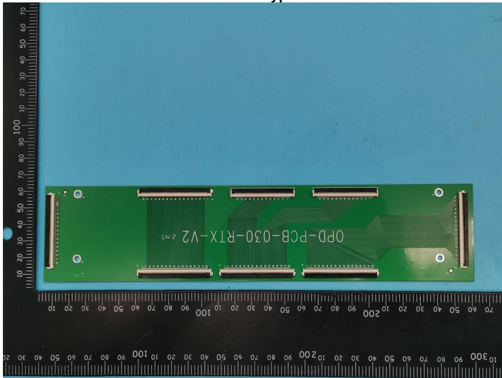
Photo 22 TP Board type A
