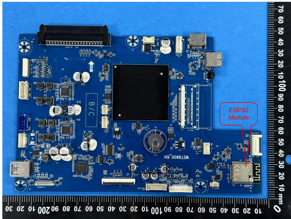
Photo 16 TP control board type B
