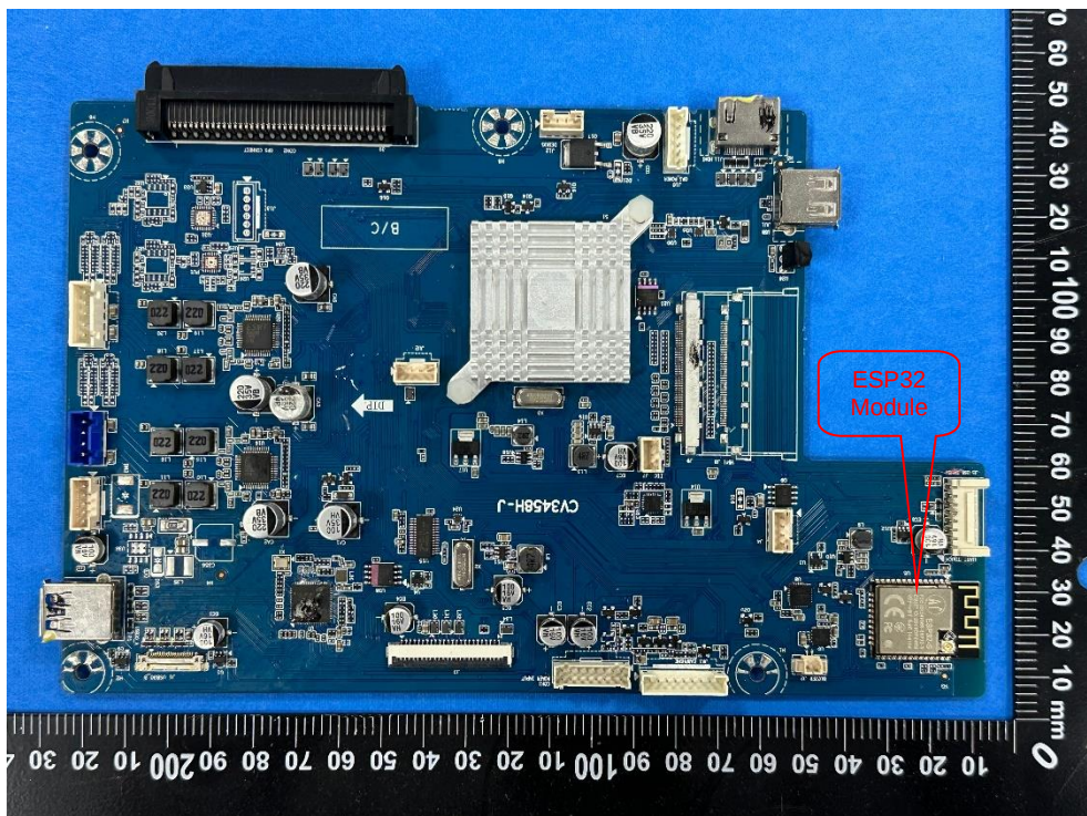
Photo 12 TP control board type A
