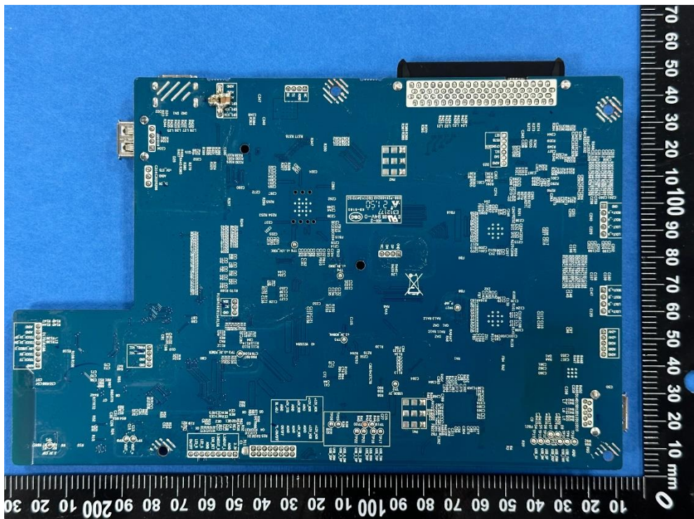
Photo 14 TP control board type A
