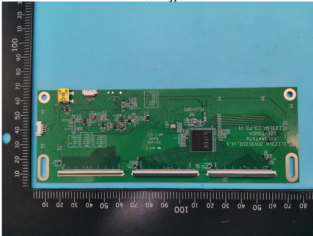
Photo 20 TP Board type A
