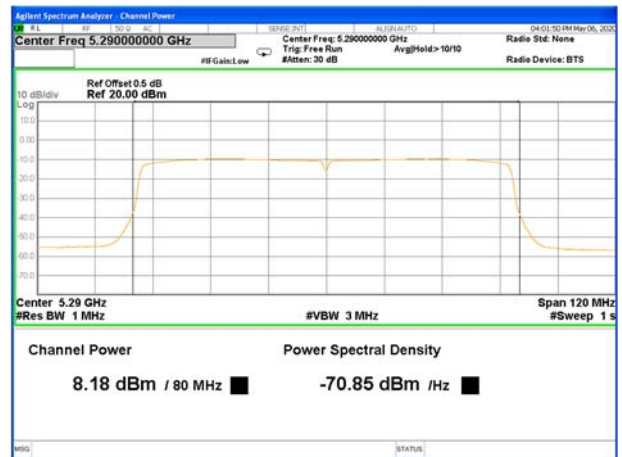
5290MHz_AV_Ant A
