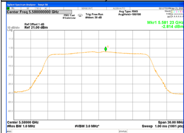
W56_11ac20_Middle_Power Spectrum Density
