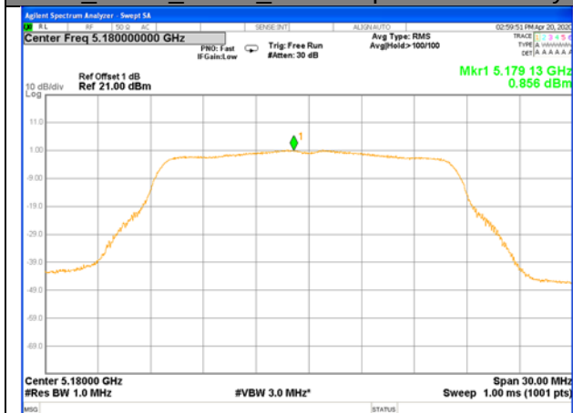
W52_11a20_Higher_Power Spectrum Density
