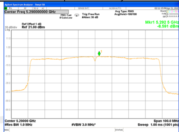
W53_11ac80_CH58(5290MHz)_Power Spectrum Density
