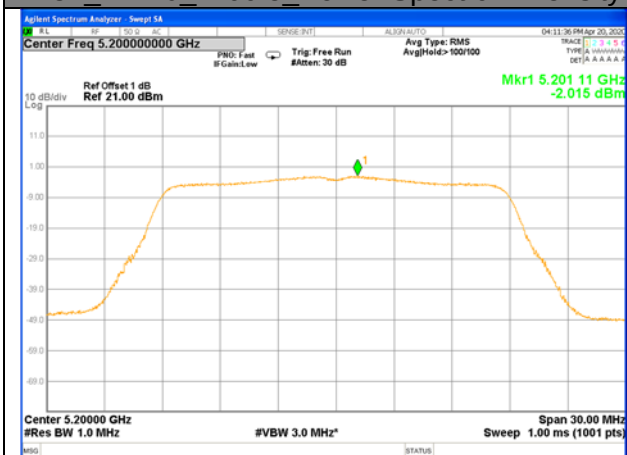
W52_11n20_Middle_Power Spectrum Density
