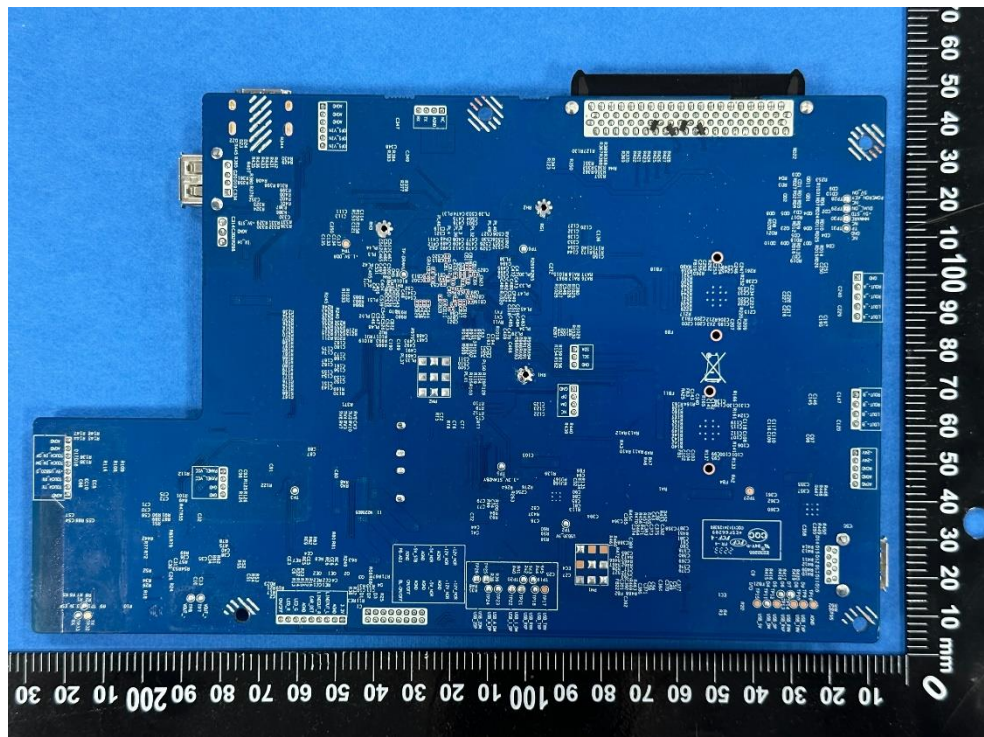
Photo 26 TP control board type B
