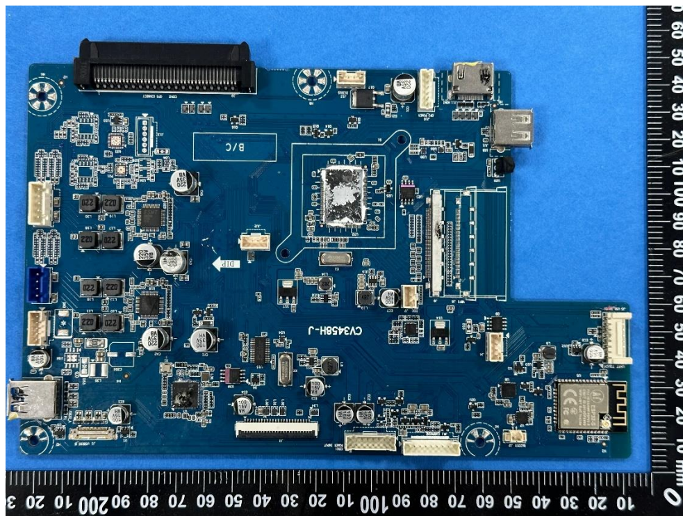
Photo 22 TP control board type A
