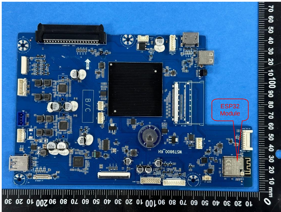
Photo 24 TP control board type B
