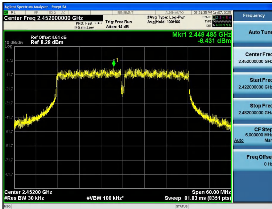
Power_Spectral_Density_NVNT_ANT1_802_11n(HT40)_2452
