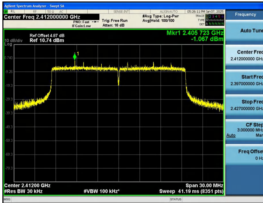
Power_Spectral_Density_NVNT_ANT1_802_11ax(HE20)_2412
