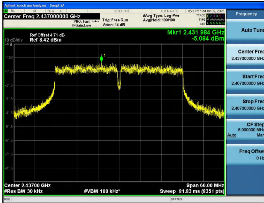
Power_Spectral_Density_NVNT_ANT1_802_11n(HT40)_2437
