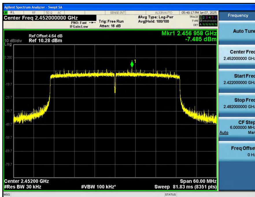
Power_Spectral_Density_NVNT_ANT1_802_11ax(HE40)_2452
