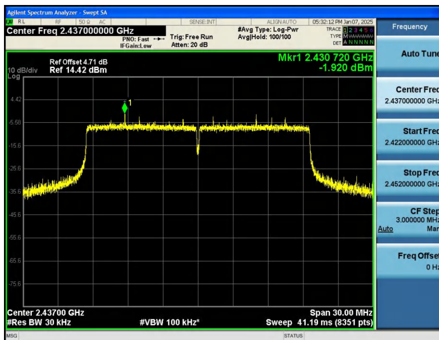
Power_Spectral_Density_NVNT_ANT1_802_11ax(HE20)_2437
