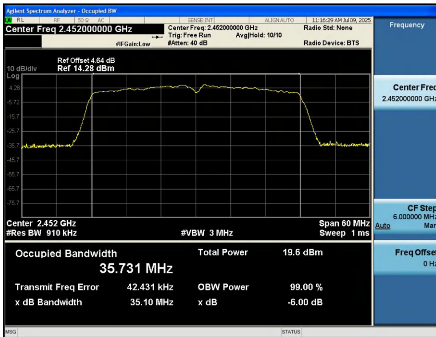
-6dB_Bandwidth_NVNT_ANT1_802_11n(HT40)_2452
