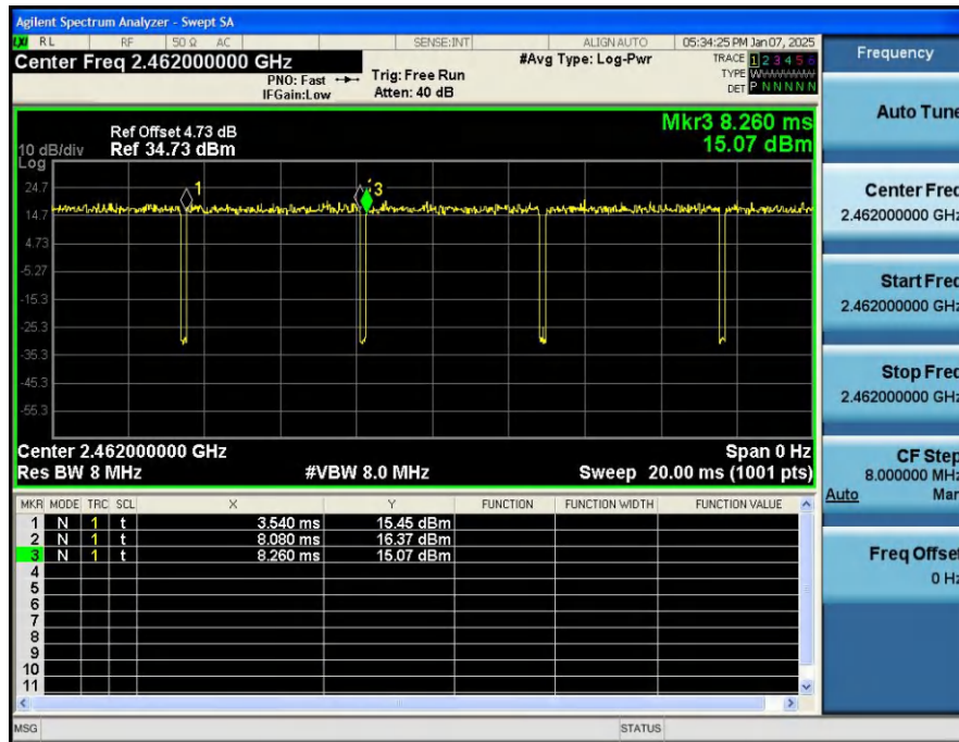
Duty_Cycle_NVNT_ANT1_802_11ax(HE20)_2462
