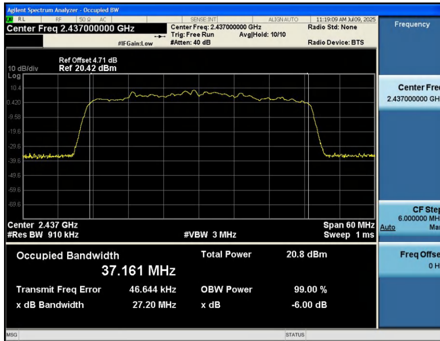
-6dB_Bandwidth_NVNT_ANT1_802_11ax(HE40)_2437
