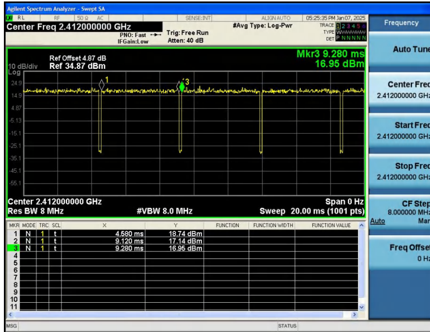
Duty_Cycle_NVNT_ANT1_802_11ax(HE20)_2412
