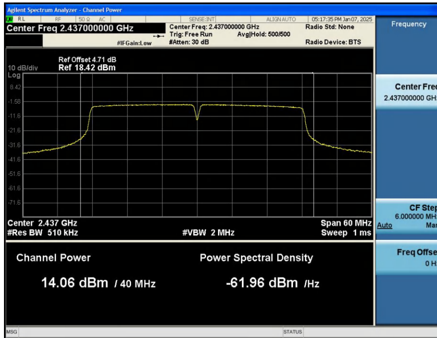
MAX_Output_Power_NVNT_ANT1_802_11n(HT40)_2437
