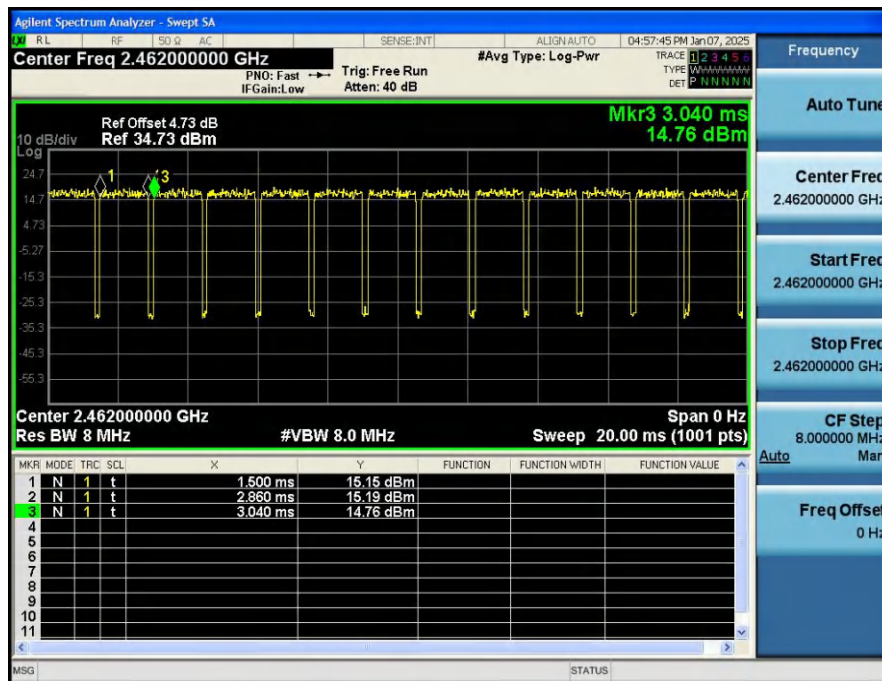
Duty_Cycle_NVNT_ANT1_802_11g_2462
