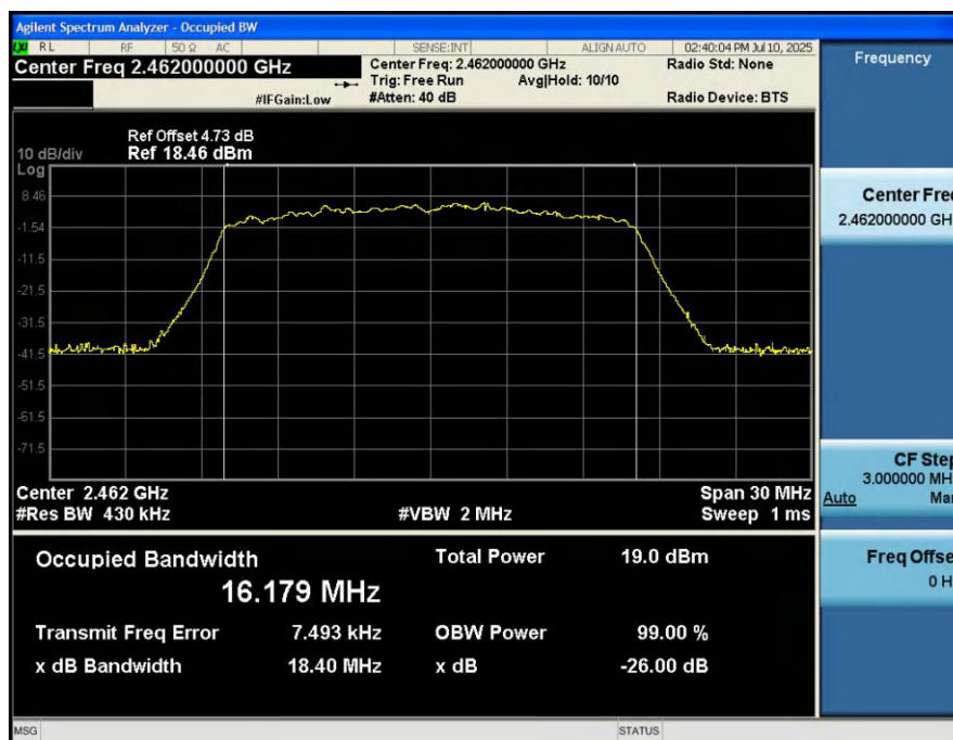
99%_Occupied_Bandwidth_NVNT_ANT1_802_11g_2462
