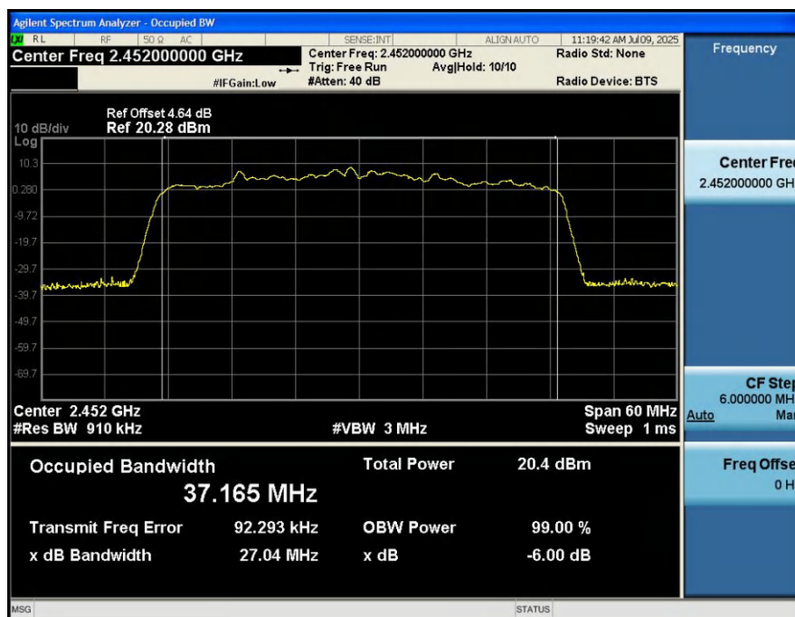
-6dB_Bandwidth_NVNT_ANT1_802_11ax(HE40)_2452
