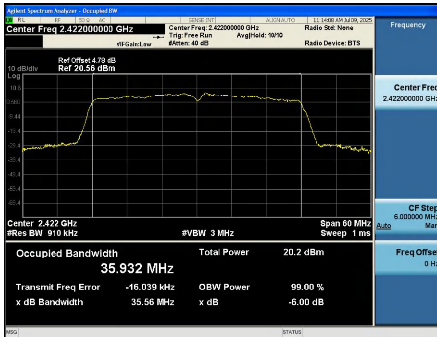
-6dB_Bandwidth_NVNT_ANT1_802_11n(HT40)_2422
