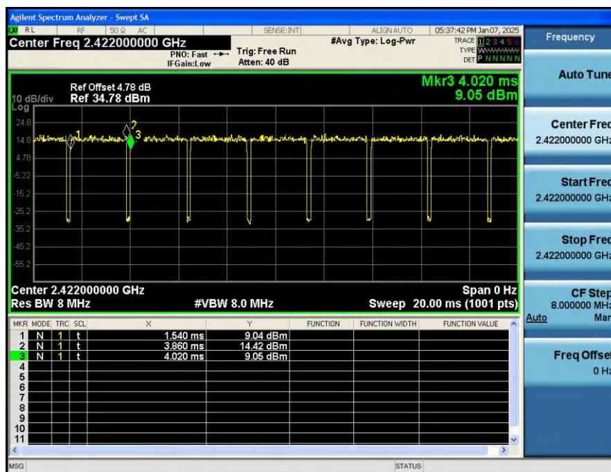
Duty_Cycle_NVNT_ANT1_802_11ax(HE40)_2422
