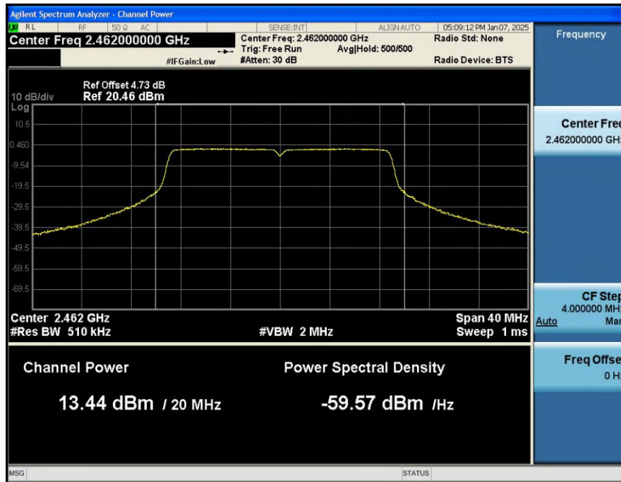
MAX_Output_Power_NVNT_ANT1_802_11n(HT20)_2462
