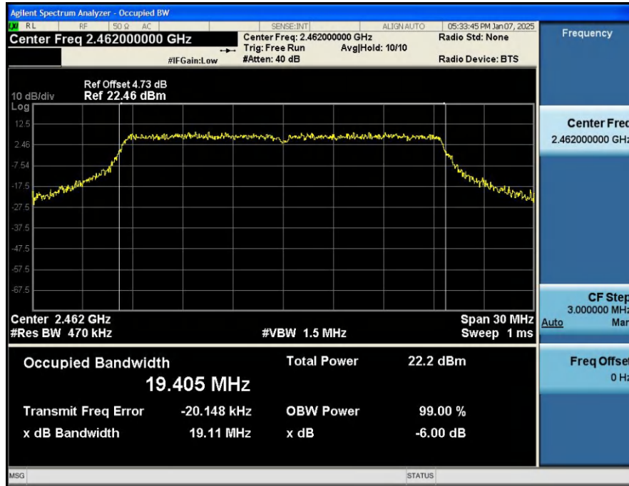
-6dB_Bandwidth_NVNT_ANT1_802_11ax(HE20)_2462
