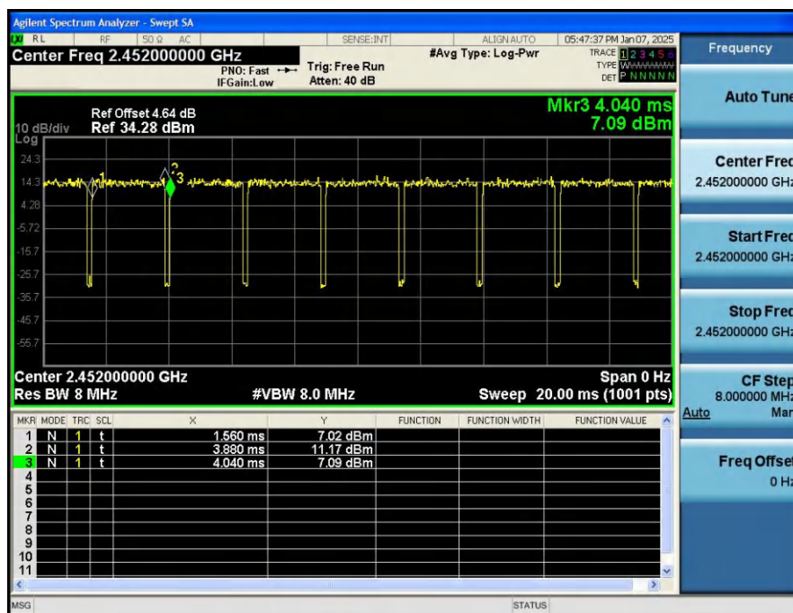
Duty_Cycle_NVNT_ANT1_802_11ax(HE40)_2452
