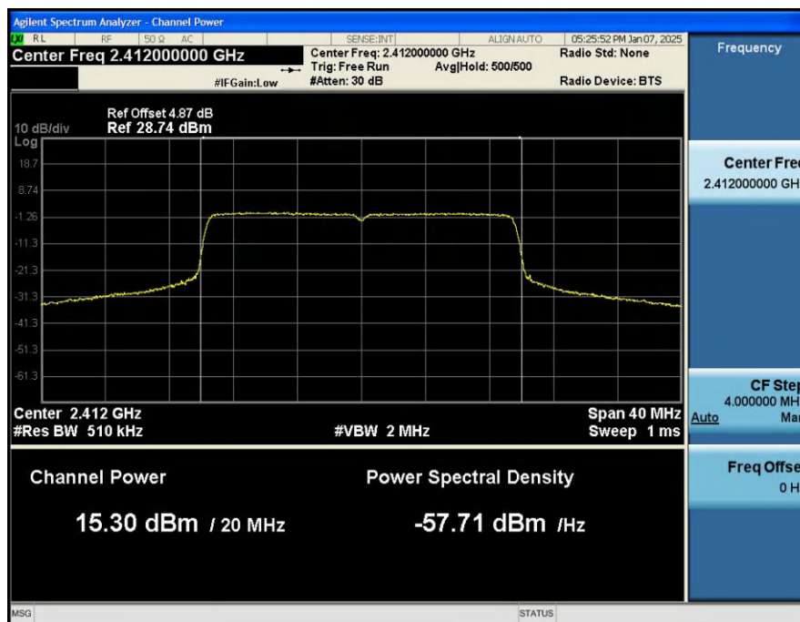
MAX_Output_Power_NVNT_ANT1_802_11ax(HE20)_2412
