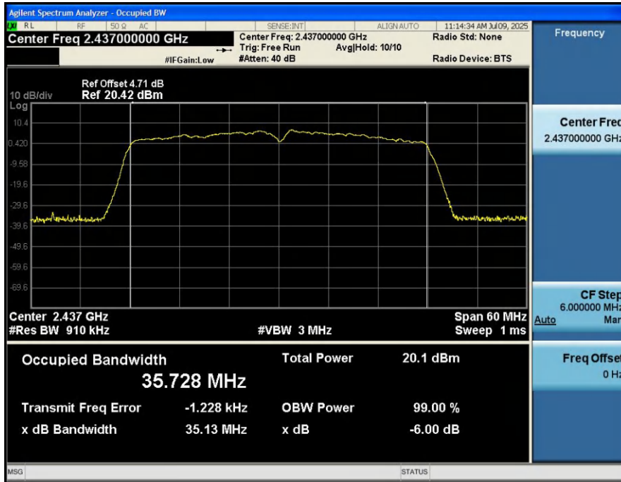
-6dB_Bandwidth_NVNT_ANT1_802_11n(HT40)_2437
