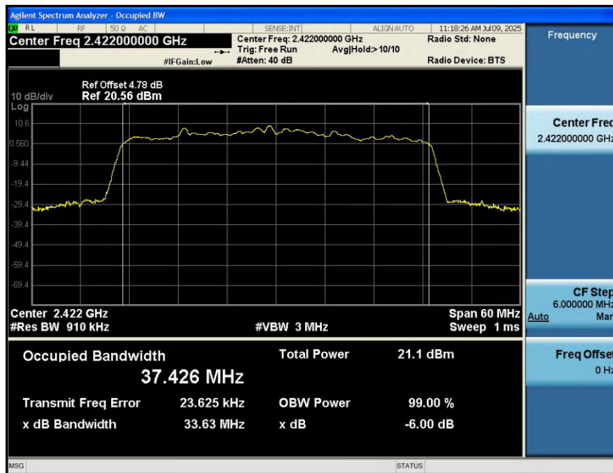
-6dB_Bandwidth_NVNT_ANT1_802_11ax(HE40)_2422
