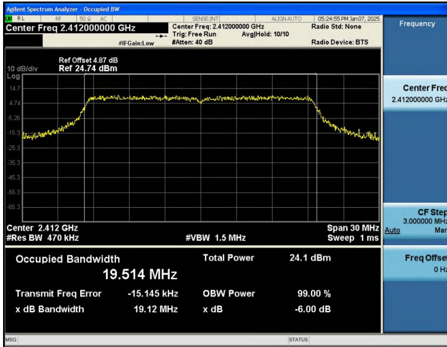
-6dB_Bandwidth_NVNT_ANT1_802_11ax(HE20)_2412
