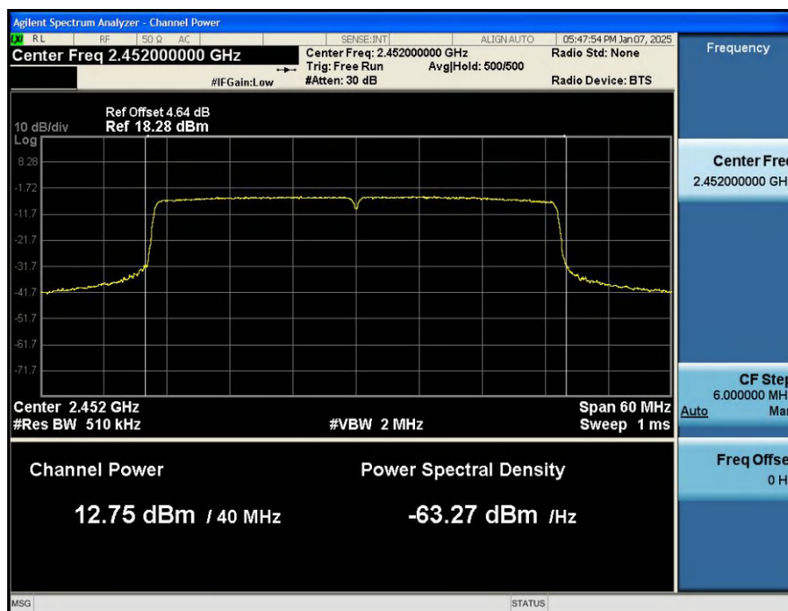
MAX_Output_Power_NVNT_ANT1_802_11ax(HE40)_2452
