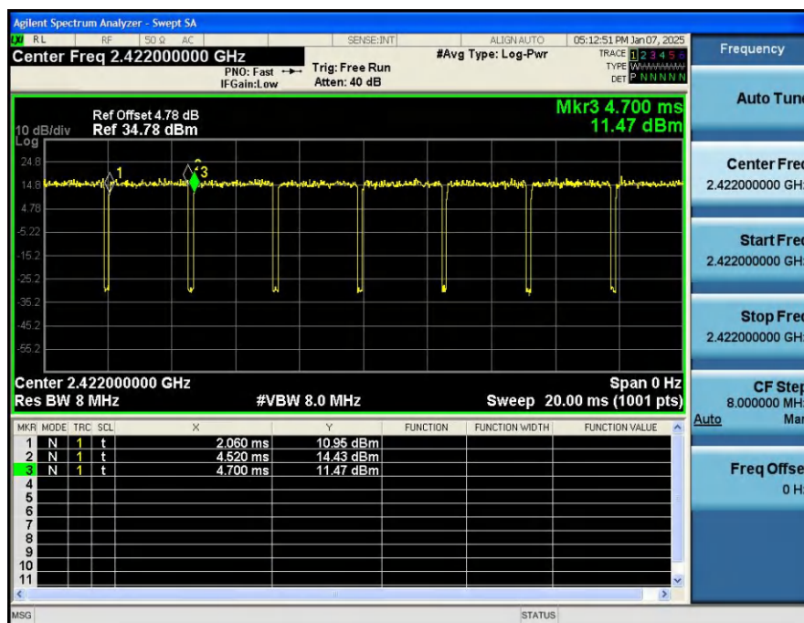
Duty_Cycle_NVNT_ANT1_802_11n(HT40)_2422
