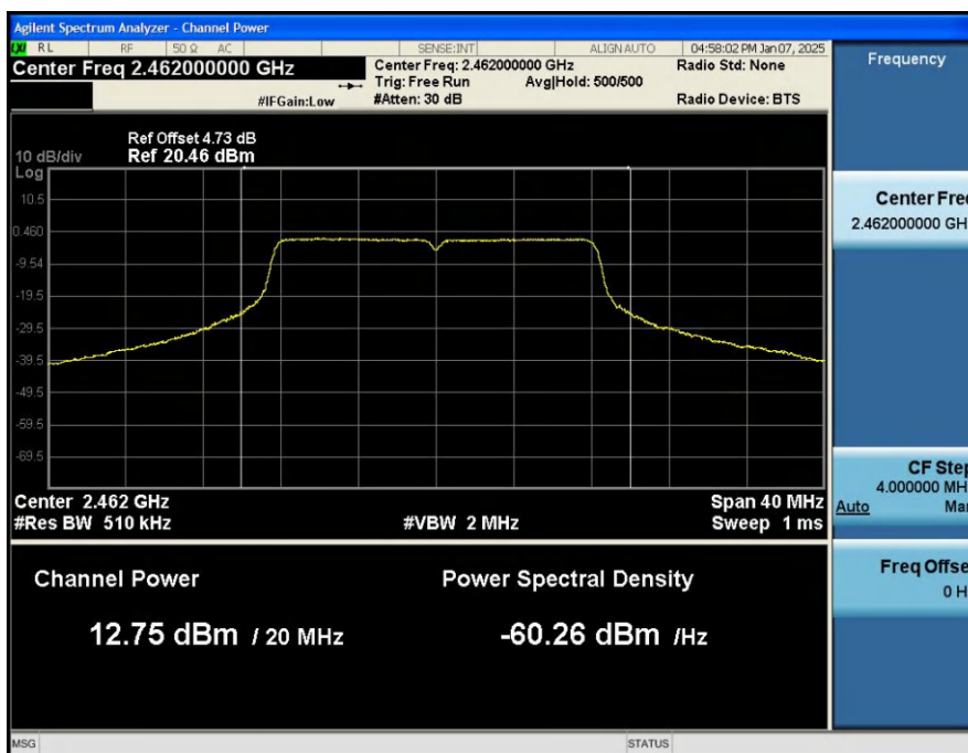
MAX_Output_Power_NVNT_ANT1_802_11g_2462
