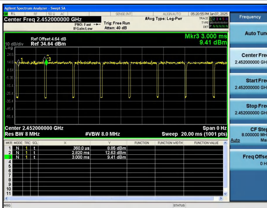
Duty_Cycle_NVNT_ANT1_802_11n(HT40)_2452
