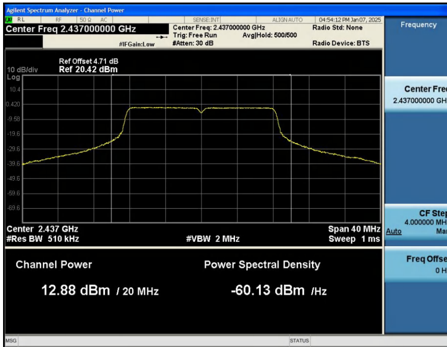
MAX_Output_Power_NVNT_ANT1_802_11g_2437
