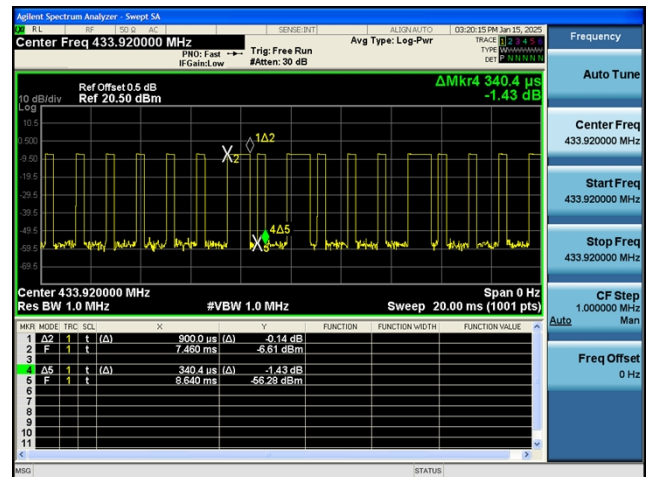
T on1
