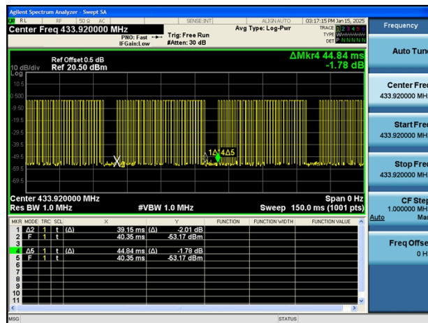
T period
