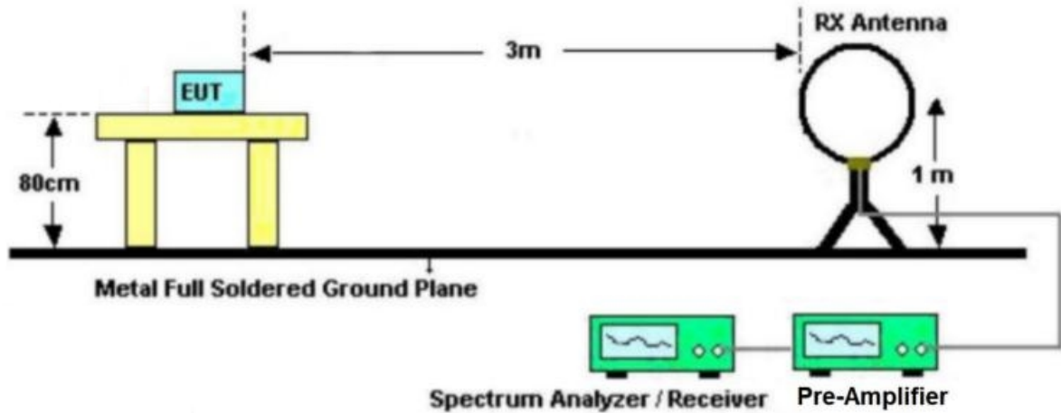
Figure 1. Below 30MHz
