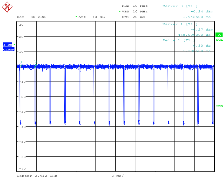
Test Graph_ IEEE802.11g Duty Cycle: 92.99%
