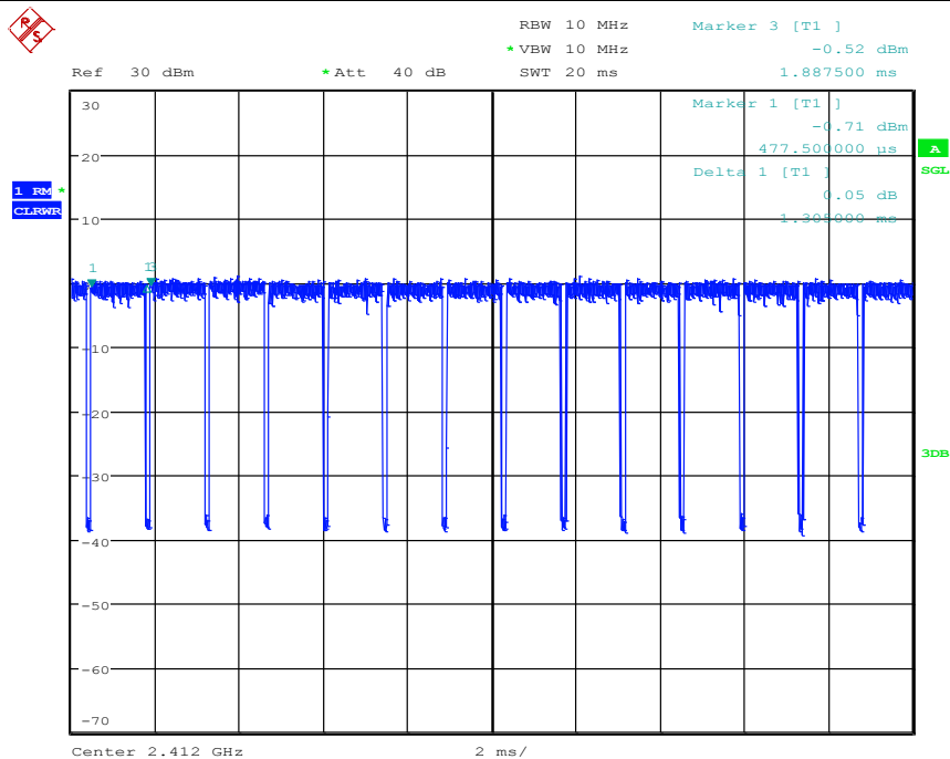
Test Graph_ IEEE802.11 n (HT20) Duty Cycle: 92.55%
