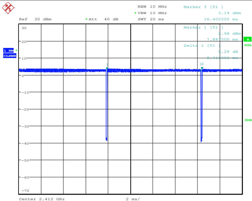
Test Graph_ IEEE802.11b Duty Cycle: 98.77%
