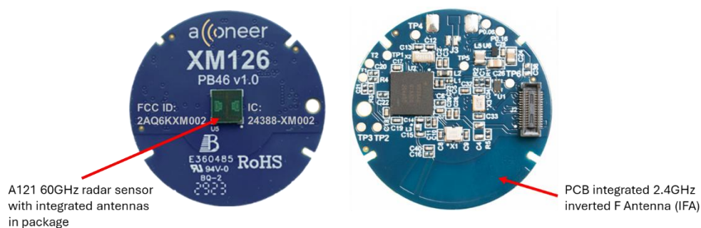
Figure 3: Frontside and backside of the XM126 module.
