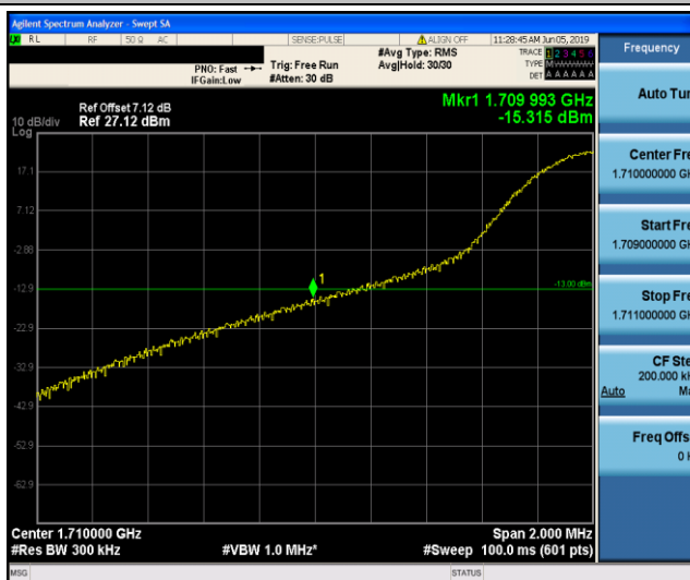
Band4_15MHz_16QAM_20025_1RB#0
