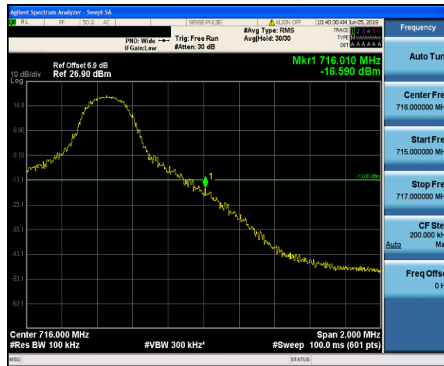
Band17_5MHz_QPSK_23825_1RB#24
