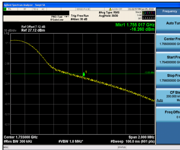
Band4_15MHz_QPSK_20325_1RB#74
