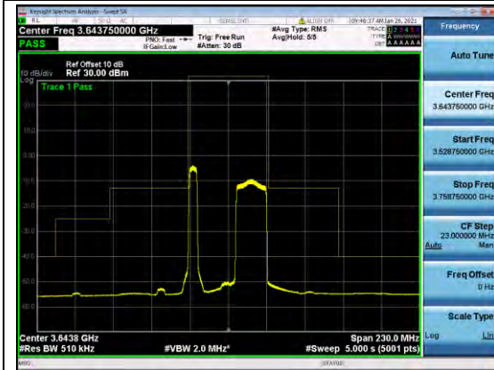
B48-NON-5-20-MASK-H-QPSK
