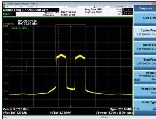
B48-NON-20-5-MASK-L-QPSK
