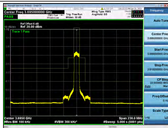
B48-10M-MASK-H-Q64
