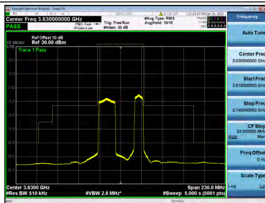
B48-NON-20-10-MASK-H-Q16
