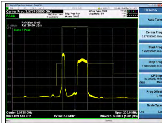
B48-NON-5-20-MASK-M-Q16
