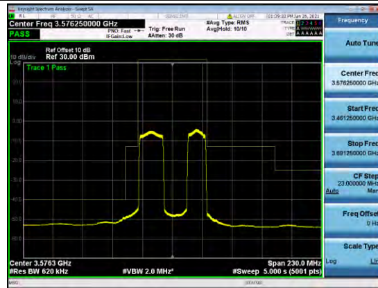
B48-NON-20-15-MASK-L-Q64
