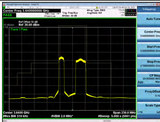
B48-NON-10-20-MASK-H-QPSK
