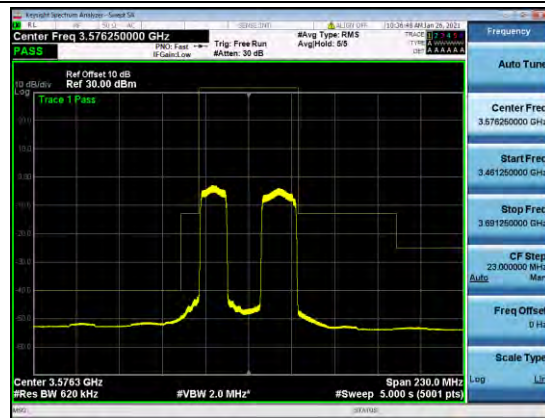
B48-NON-15-20-MASK-M-Q16
