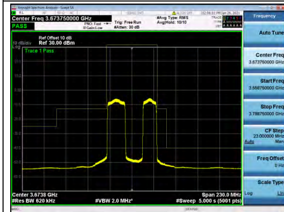
B48-NON-20-20-MASK-L-QPSK
