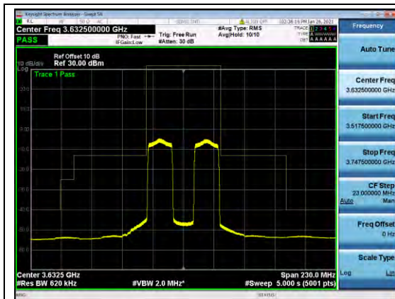
B48-NON-20-20-MASK-H-QPSK
