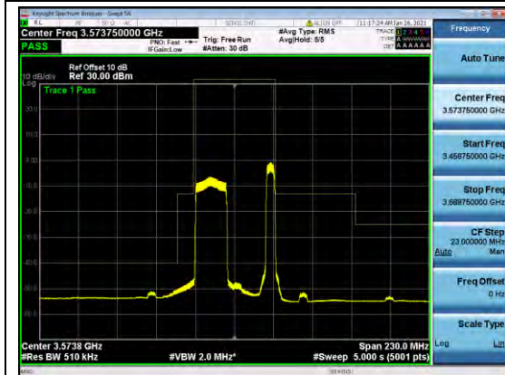
B48-NON-20-5-MASK-M-QPSK
