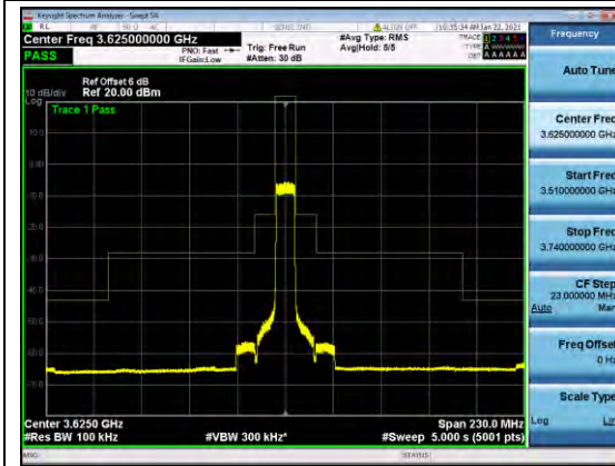
B48-10M-MASK-M-Q64
