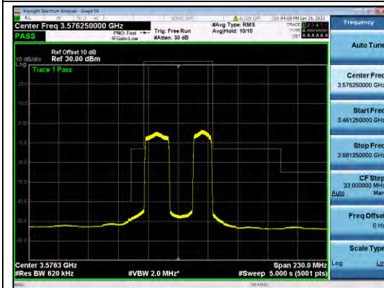
B48-NON-20-15-MASK-M-QPSK
