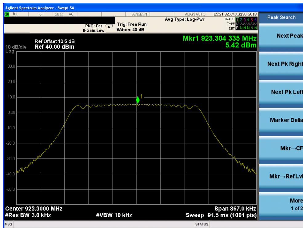
Power spectral density plot on channel 72
