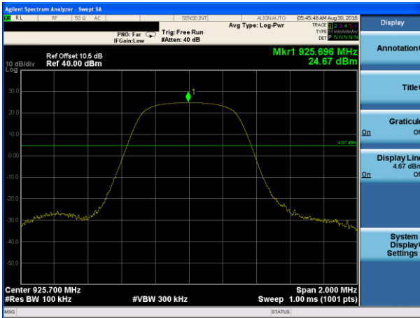
GFSK on channel 76
