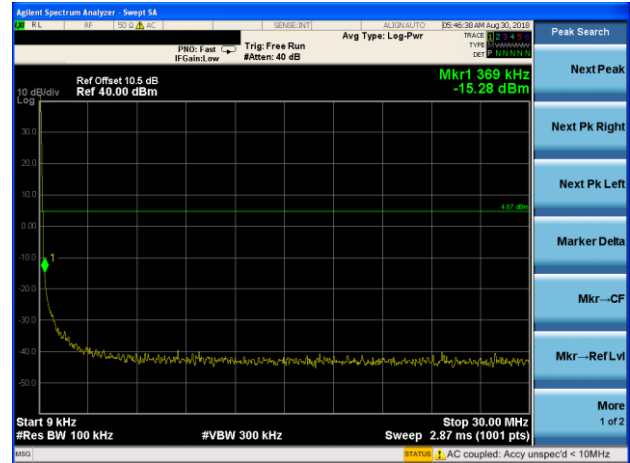
GFSK on channel 76
