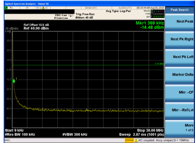
GFSK on channel 72
