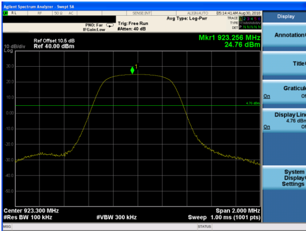
GFSK on channel 72
