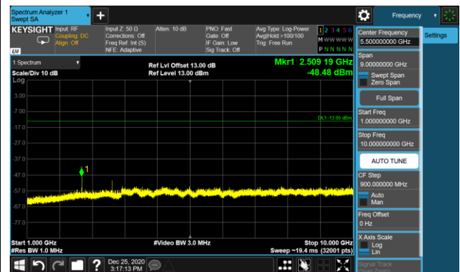
LTE Band 5 16QAM 3MHz CH20525 1RB#7_1GHz-10GHz
