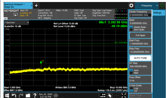
LTE Band 5 16QAM 3MHz CH20635 1RB#7_1GHz-10GHz
