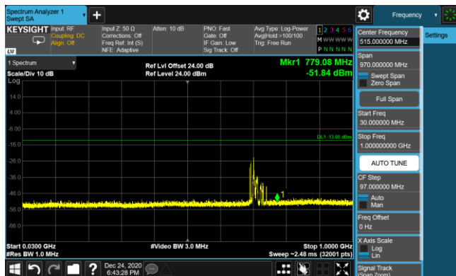
LTE Band 12 16QAM 5MHz CH23155 1RB#12_30MHz-1GHz
