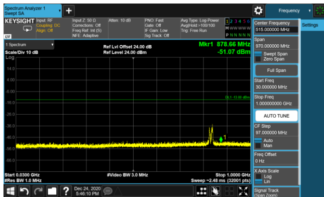
LTE Band 5 16QAM 5MHz CH20525 1RB#12_30MHz-1GHz
