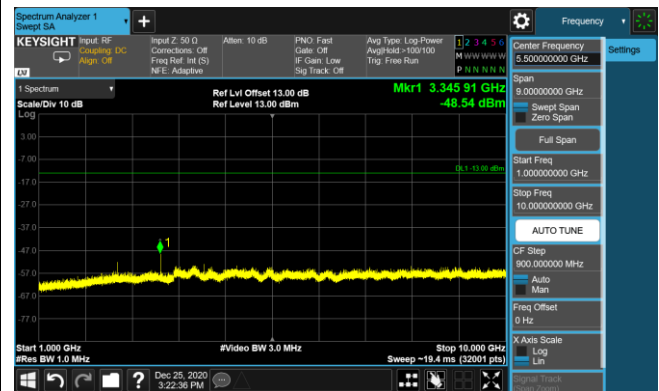
LTE Band 5 16QAM 5MHz CH20525 1RB#12_1GHz-10GHz
