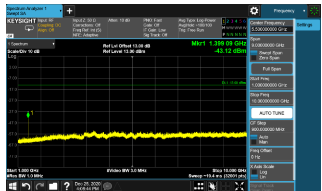
LTE Band 12 16QAM 3MHz CH23025 1RB#7_1GHz-10GHz
