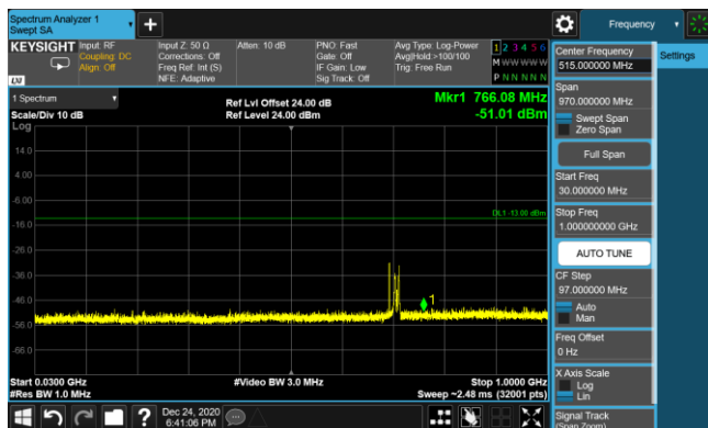
LTE Band 12 16QAM 3MHz CH23165 1RB#7_30MHz-1GHz
