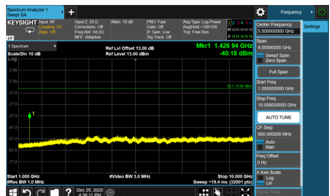
LTE Band 12 16QAM 5MHz CH23155 1RB#12_1GHz-10GHz
