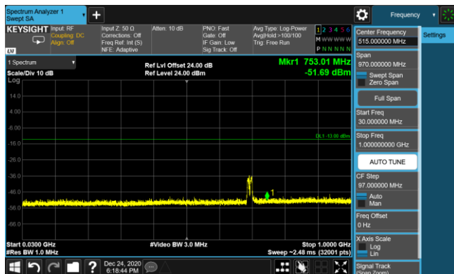
LTE Band 12 16QAM 5MHz CH23035 1RB#12_30MHz-1GHz
