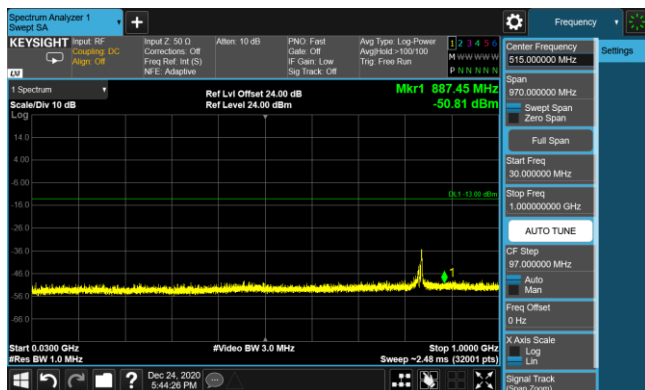
LTE Band 5 16QAM 3MHz CH20525 1RB#7_30MHz-1GHz
