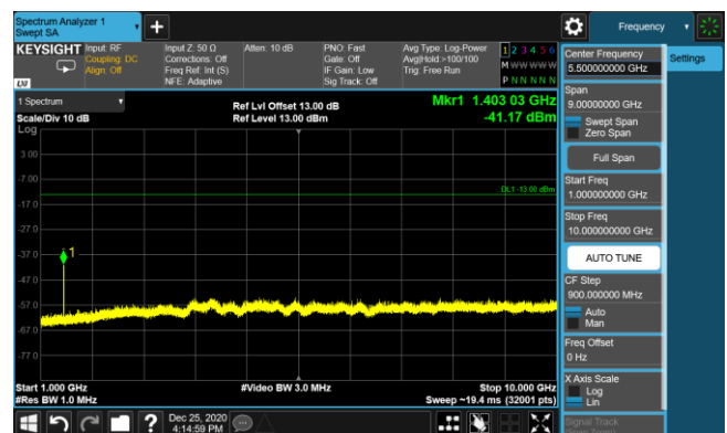
LTE Band 12 16QAM 5MHz CH23035 1RB#12_1GHz-10GHz
