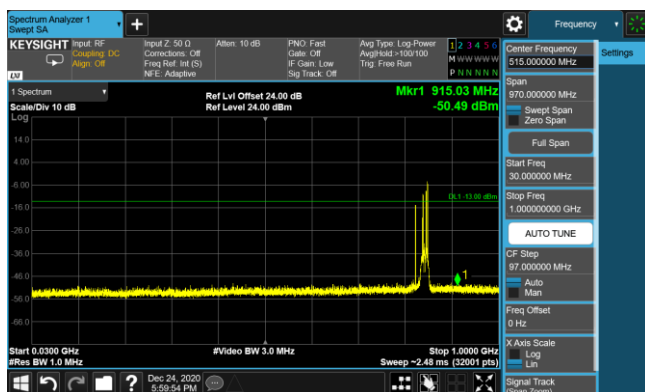
LTE Band 5 16QAM 5MHz CH20625 1RB#12_30MHz-1GHz
