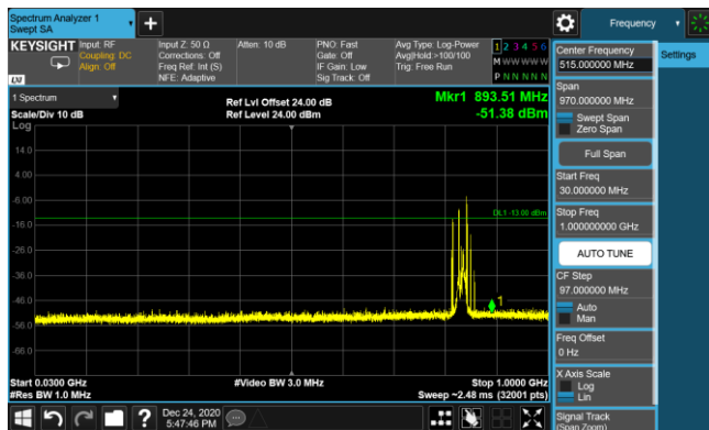
LTE Band 5 16QAM 5MHz CH20525 1RB#12_30MHz-1GHz
