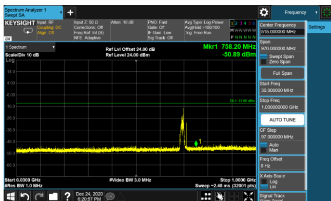
LTE Band 12 16QAM 5MHz CH23035 1RB#12_30MHz-1GHz
