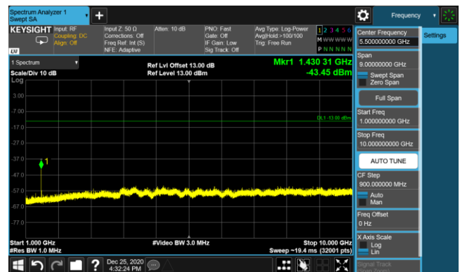
LTE Band 12 16QAM 3MHz CH23165 1RB#7_1GHz-10GHz
