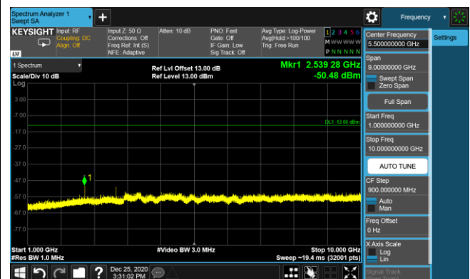
LTE Band 5 16QAM 5MHz CH20625 1RB#12_1GHz-10GHz
