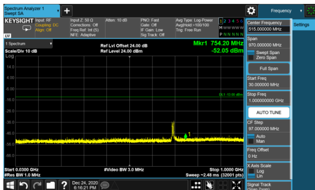
LTE Band 12 16QAM 3MHz CH23025 1RB#7_30MHz-1GHz
