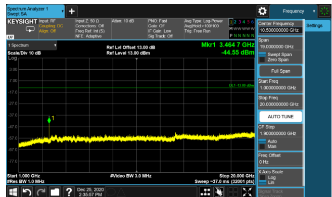
LTE Band 4 16QAM 3MHz CH20175 1RB#7_1GHz-20GHz
