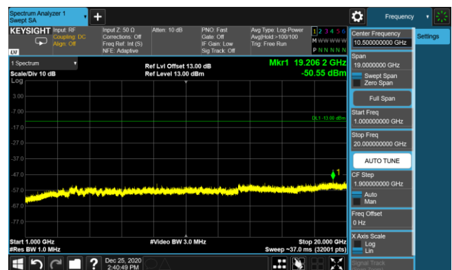
LTE Band 4 16QAM 5MHz CH20175 1RB#12_1GHz-20GHz
