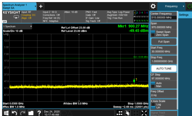
LTE Band 4 16QAM 5MHz CH20175 1RB#12_30MHz-1GHz
