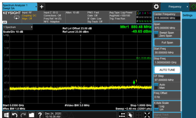
LTE Band 4 16QAM 3MHz CH20175 1RB#7_30MHz-1GHz
