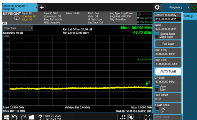
LTE Band 4 16QAM 5MHz CH20175 1RB#12_30MHz-1GHz
