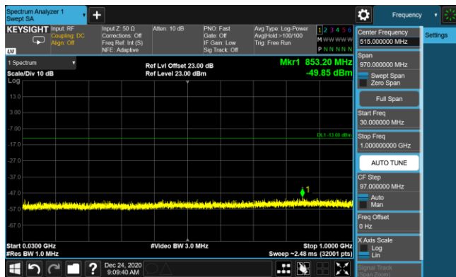
LTE Band 2 16QAM 5MHz CH18900 1RB#12_30MHz-1GHz
