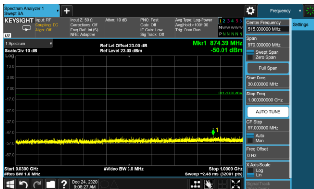
LTE Band 2 16QAM 3MHz CH18900 1RB#7_30MHz-1GHz
