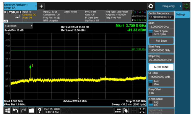
LTE Band 2 16QAM 5MHz CH18900 1RB#12_1GHz-20GHz
