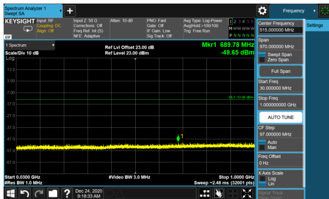
LTE Band 2 16QAM 5MHz CH18900 1RB#12_30MHz-1GHz
