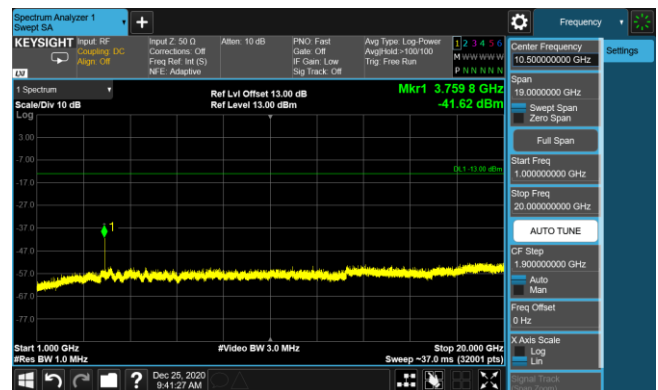
LTE Band 2 16QAM 3MHz CH18900 1RB#7_1GHz-20GHz
