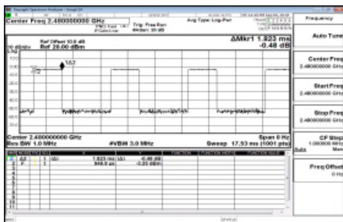
Dwell Time_8DPSK_3M_DH3_2480MHz
