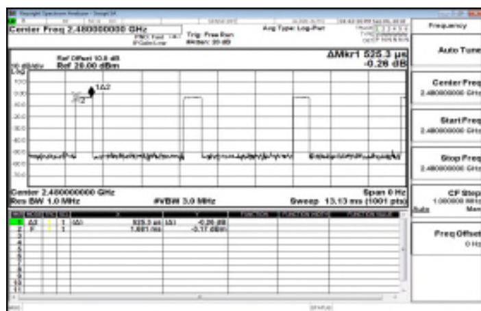
Dwell Time_π4DQPSK_2M_DH1_2480MHz
