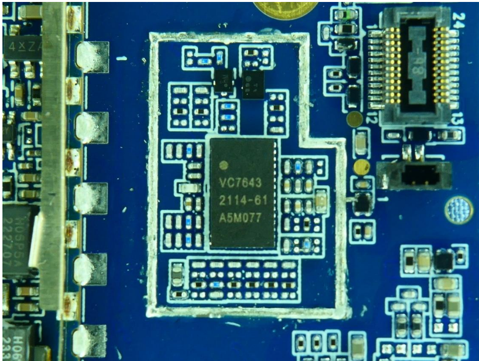
(27) EUT Photo
