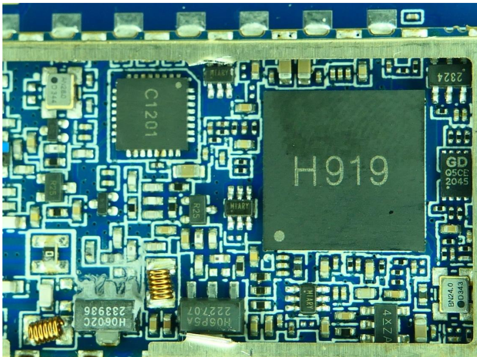
(26) EUT Photo
